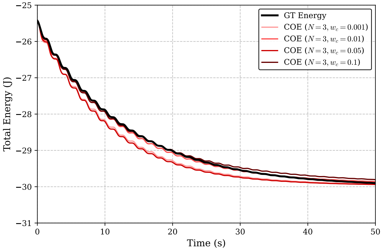
Total Energy (50.0s Rollout) - Effect of Consensus Weight ( N=3 )
