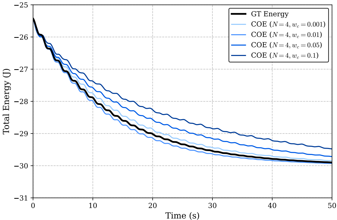
Total Energy (50.0s Rollout) - Peak Performance ( N=4 )
