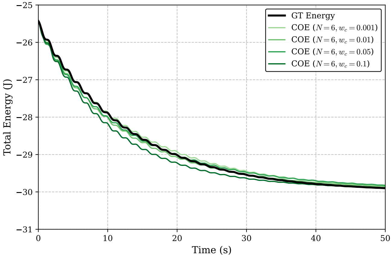
Total Energy (50.0s Rollout) - Effect of Consensus Weight ( N=6 )
