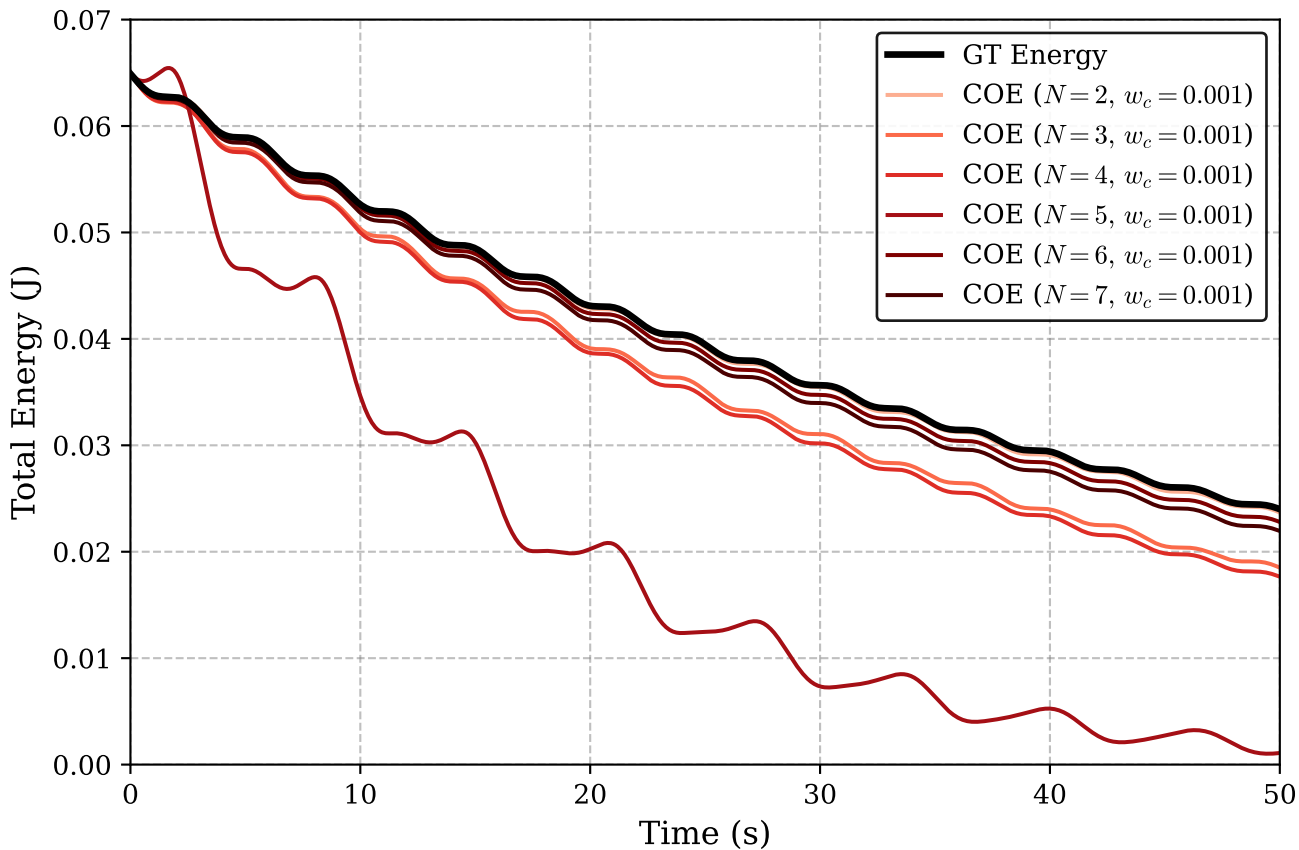
Total Energy (50.0s Rollout) - Scaling N at w_c = 0.001
