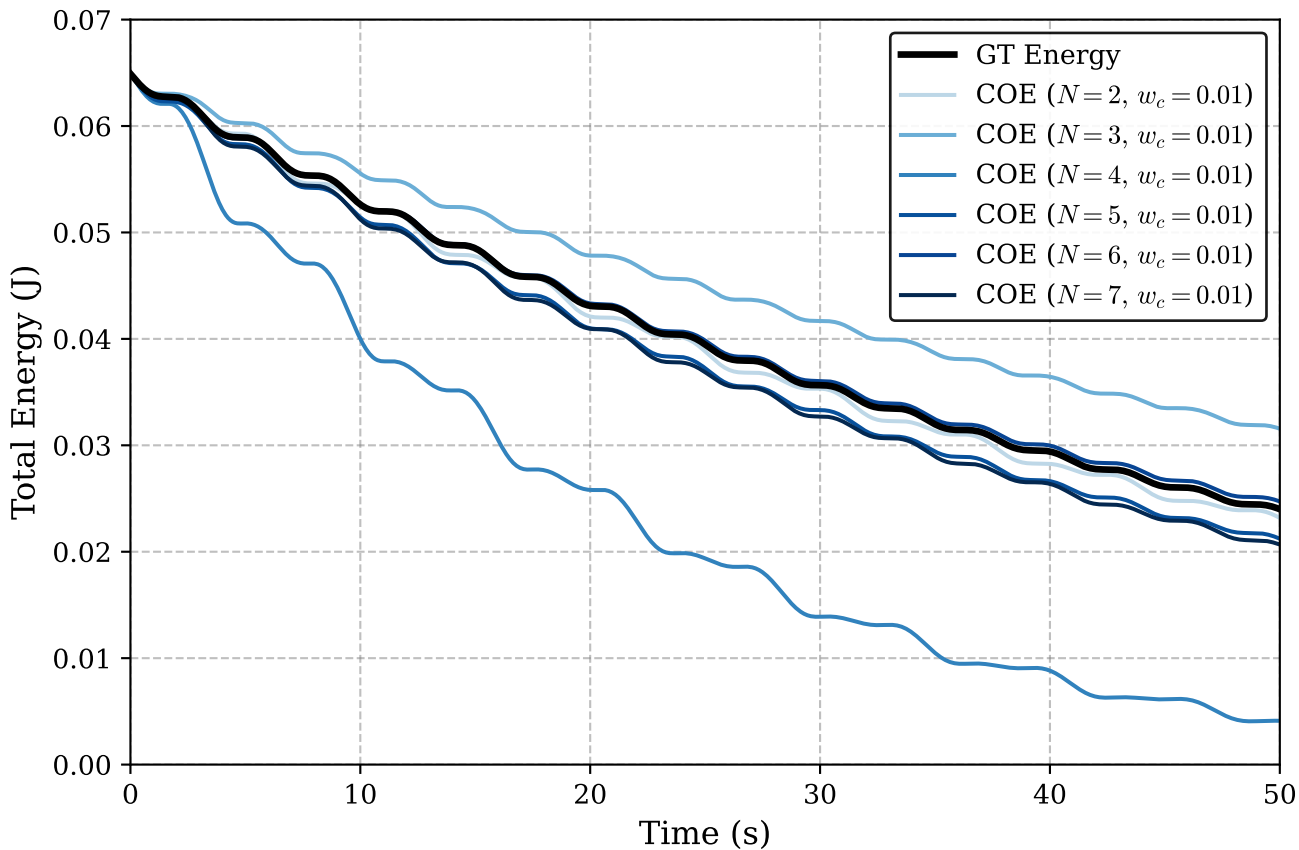
Total Energy (50.0s Rollout) - Scaling N at w_c = 0.01
