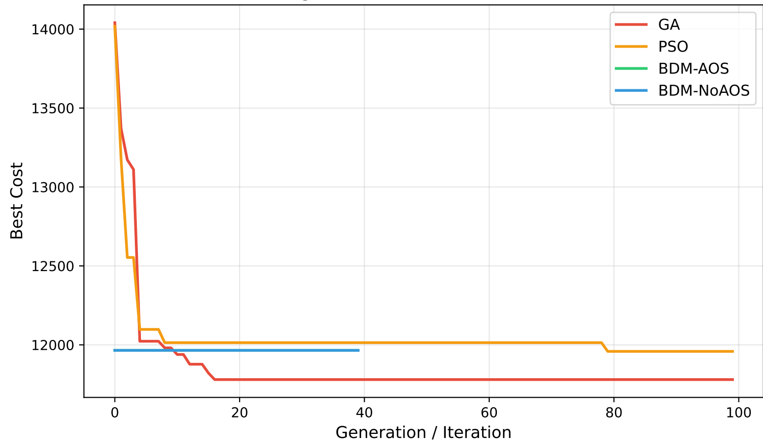
Convergence on S10 (mean over 3 seeds)
