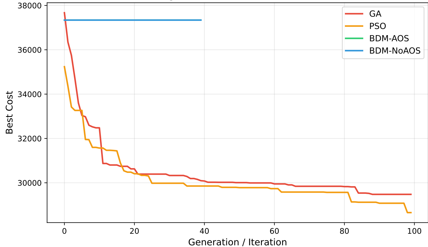
Convergence on S20 (mean over 3 seeds)
