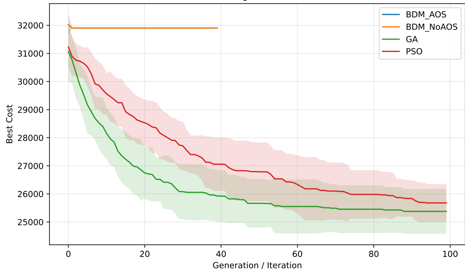
Convergence — S20
