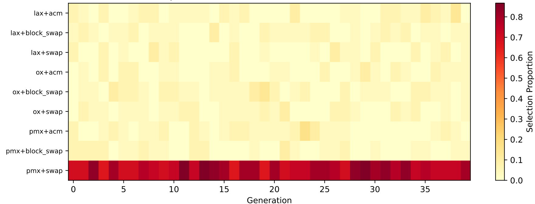
Operator Selection Over Generations — S10
