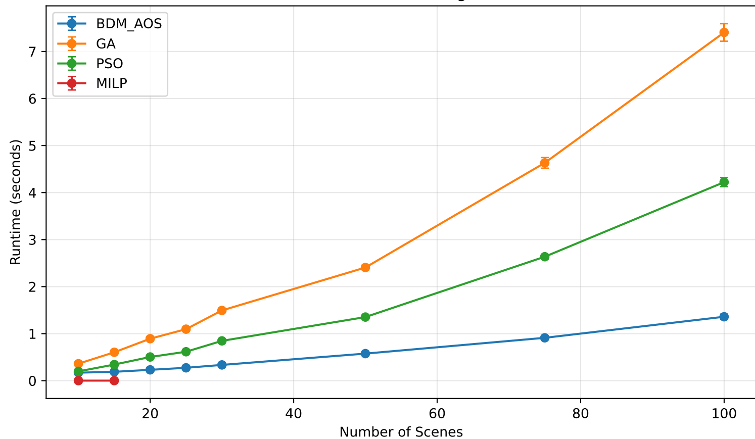
Runtime Scaling
