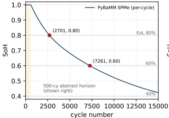
(a) EVE_0004 anchor \theta — full 15,000-cy PyBaMM SPMe run 45.4 min wall, min SoH 0.423
