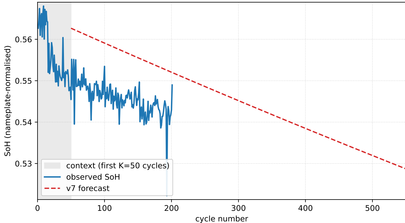
REPT_0031 — v7 held-out forecast (in-coverage RMSE = 1.21 pp, n_covered=152)
