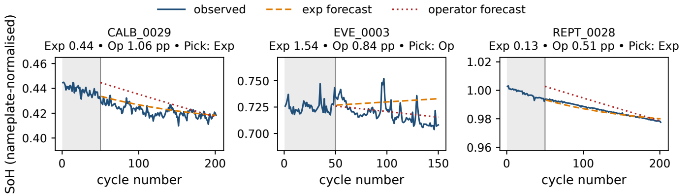
Figure 2: Forecasts evaluated against measured post-context SoH for three external cells. Grey shading denotes the K=50 context window; orange dashed and red dotted lines show exponential and neural-operator forecasts, respectively. Panels use independent y-axis ranges.
