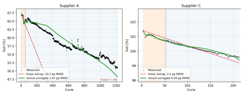
Figure 1: Best-tracking cell per supplier (ranked by peak deviation across the full held-out window). K=50 training window in orange, held-out in blue. On the deep-second-life supplier-A cell, linear-slope extrapolation (red-dashed) exits the frame while the neural surrogate (green) tracks measured across 1200+ cycles; on the light-fade supplier-C cell both methods sit under 0.2 pp.
