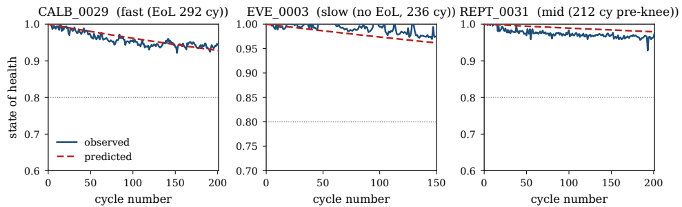
Figure 1: Per-cell SoH predictions on three held-out cells (CALB_0029, EVE_0003, REPT_0031). Blue: observed cycling. Red dashed: operator prediction from a nearest-supplier-anchor \theta prior. Dotted line: end-of-life threshold ( \text{SoH} = 0.80 ). Per-cell in-window SoH RMSE: CALB_0029 = 1.05 pp, EVE_0003 = 1.76 pp, REPT_0031 = 1.69 pp; cross-supplier RMSE std = 0.32 pp.
