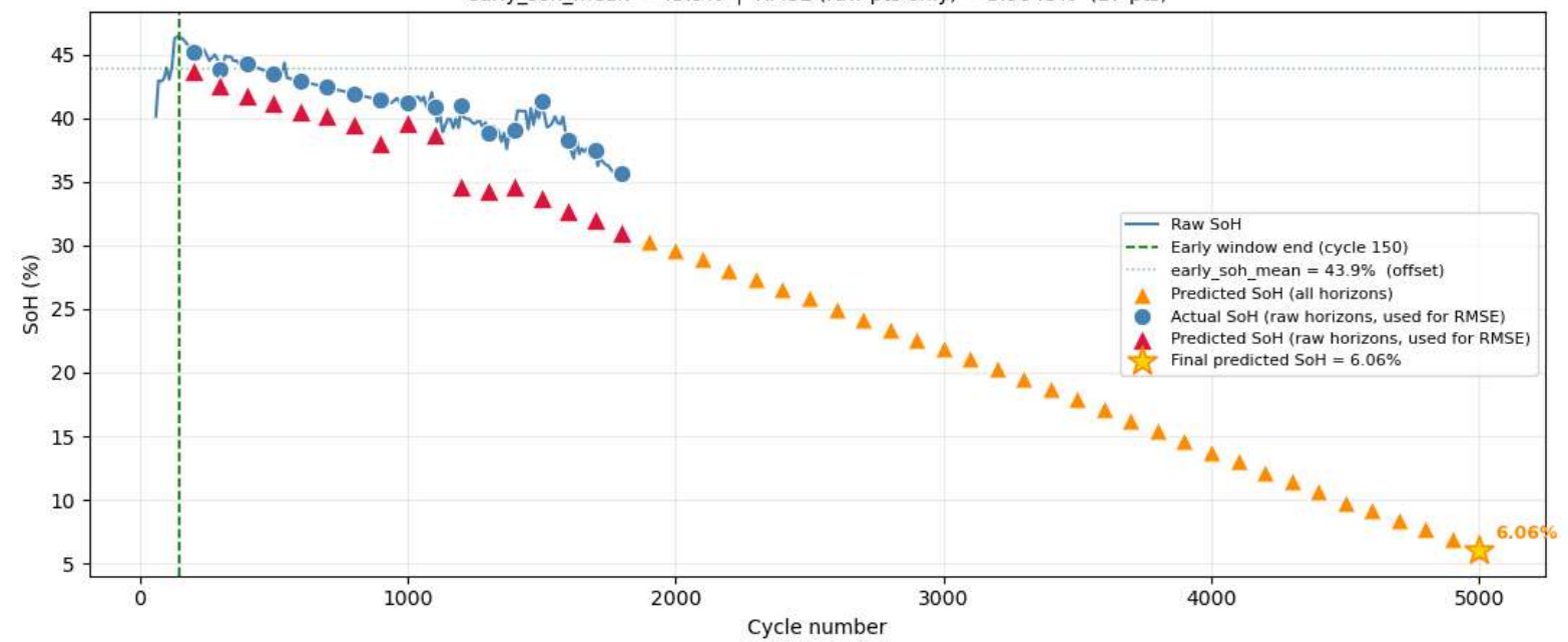
Cell 27 — Raw SoH vs Predictions early_soh_mean = 43.9% | RMSE (raw pts only) = 3.9643% (17 pts)
