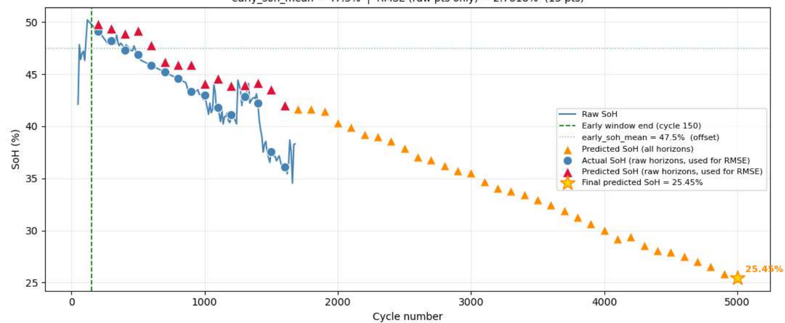
Cell 22 — Raw SoH vs Predictions early_soh_mean = 47.5% | RMSE (raw pts only) = 2.7818% (15 pts)
