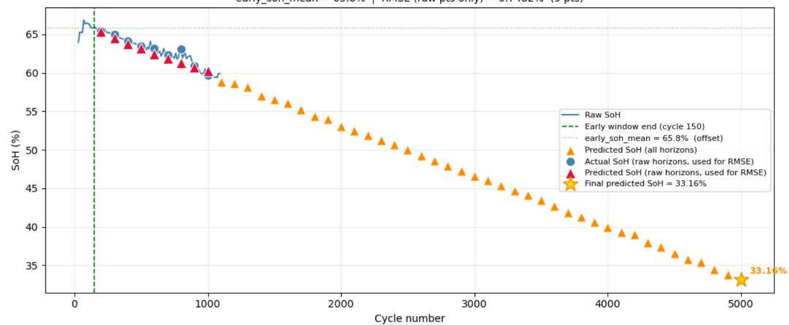
Cell 6 — Raw SoH vs Predictions early_soh_mean = 65.8% | RMSE (raw pts only) = 0.7482% (9 pts)
