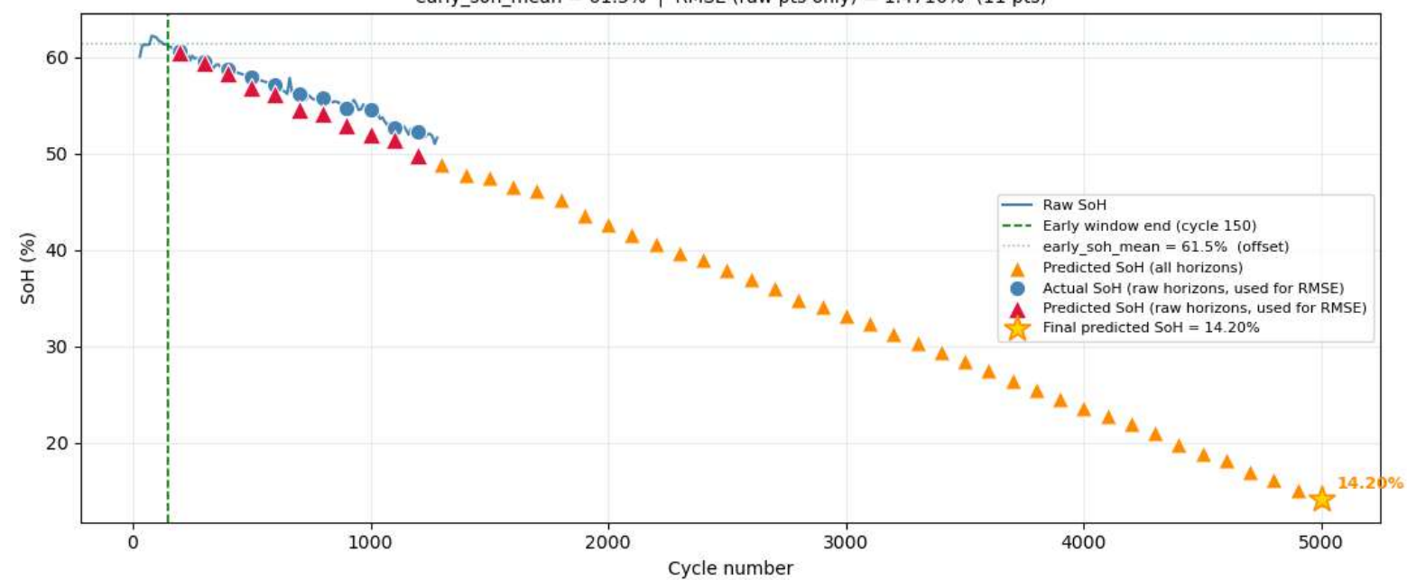
Cell 14 — Raw SoH vs Predictions early_soh_mean = 61.5% | RMSE (raw pts only) = 1.4716% (11 pts)
