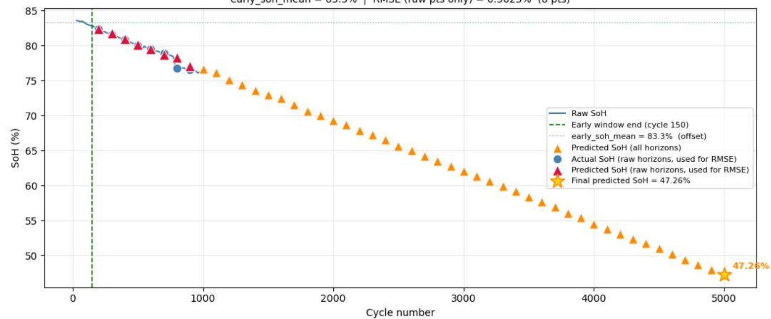
Cell 15 — Raw SoH vs Predictions early_soh_mean = 83.3% | RMSE (raw pts only) = 0.5625% (8 pts)
