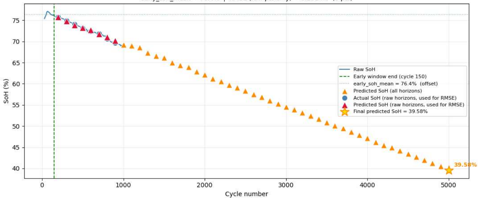
Cell 9 — Raw SoH vs Predictions early_soh_mean = 76.4% | RMSE (raw pts only) = 0.2914% (8 pts)
