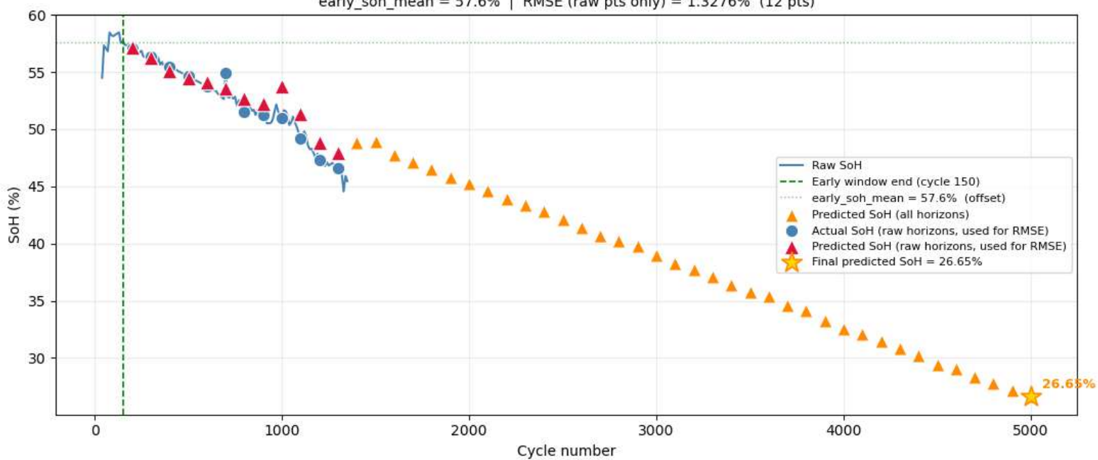
Cell 12 — Raw SoH vs Predictions early_soh_mean = 57.6% | RMSE (raw pts only) = 1.3276% (12 pts)
