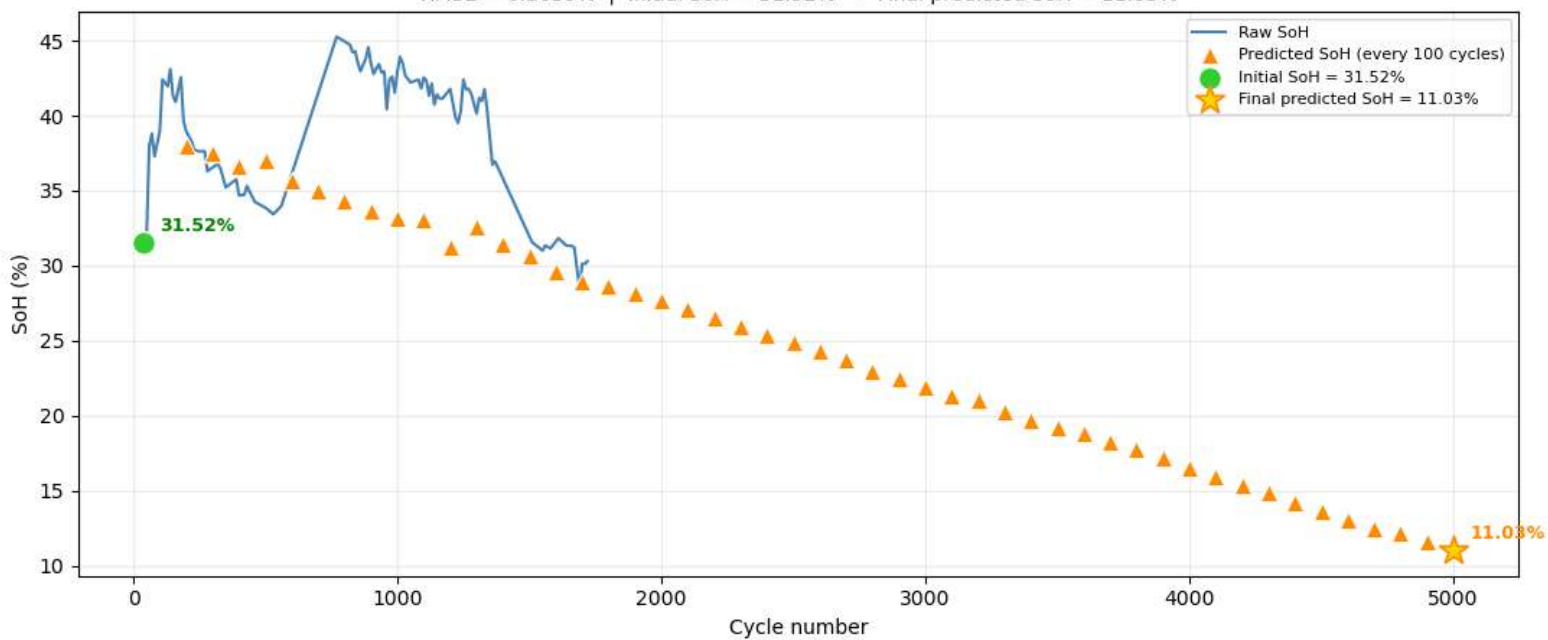
Cell 16 — Raw SoH vs Predictions RMSE = 6.3639% | Initial SoH = 31.52% → Final predicted SoH = 11.03%
