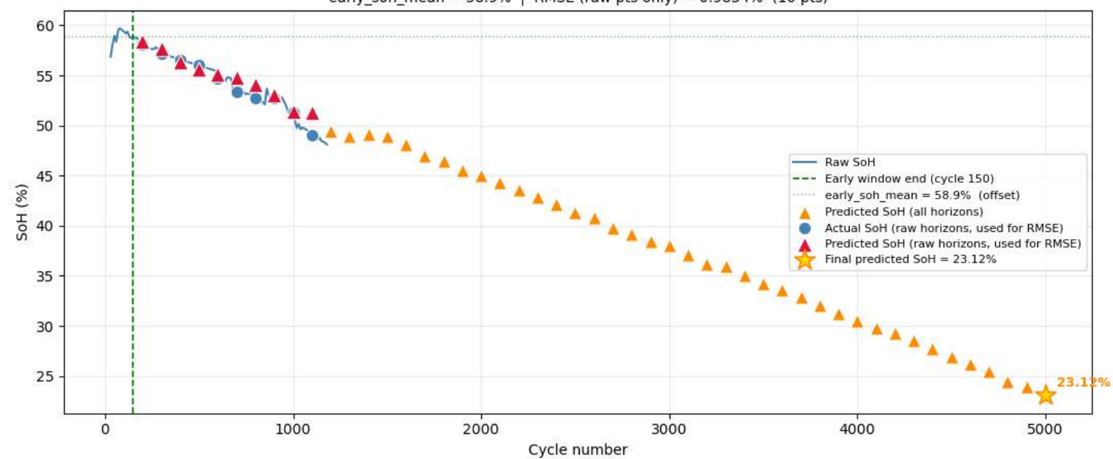
Cell 7 — Raw SoH vs Predictions early_soh_mean = 58.9% | RMSE (raw pts only) = 0.9834% (10 pts)
