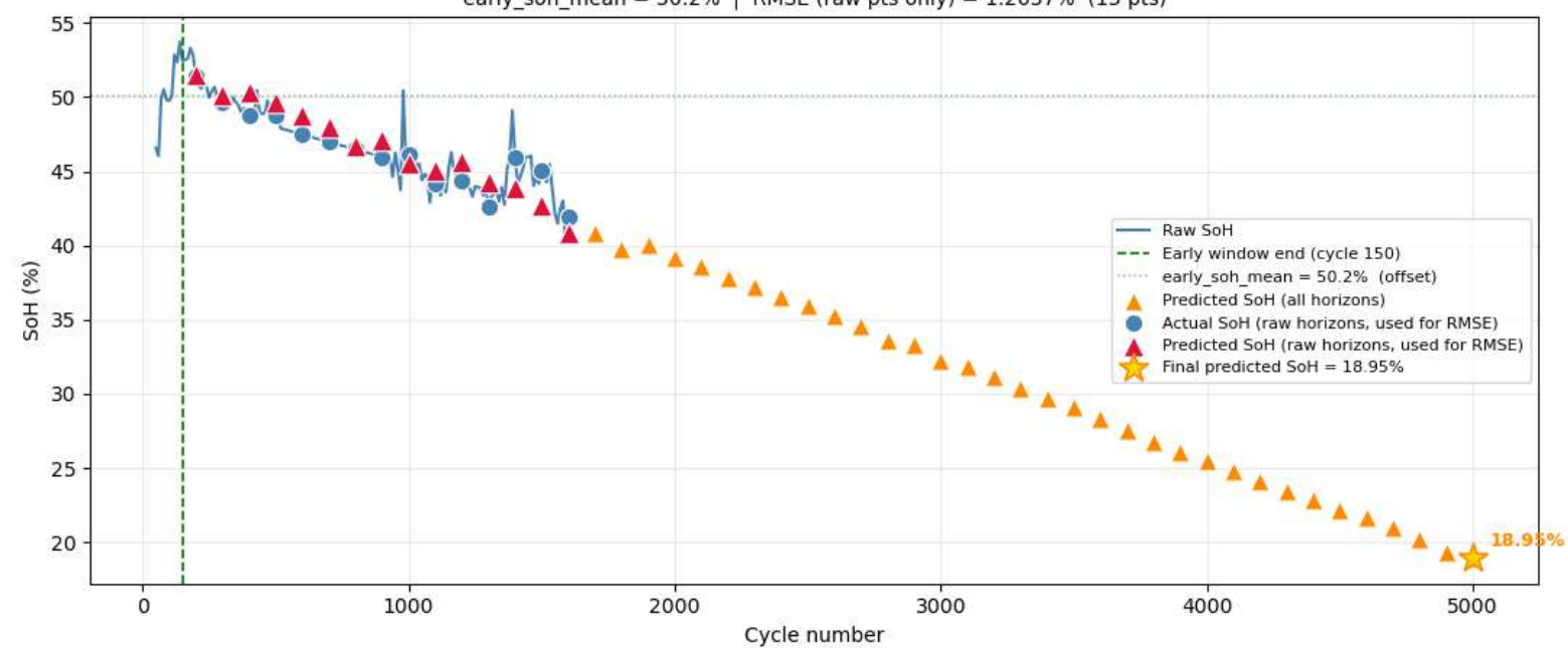
Cell 26 — Raw SoH vs Predictions early_soh_mean = 50.2% | RMSE (raw pts only) = 1.2637% (15 pts)
