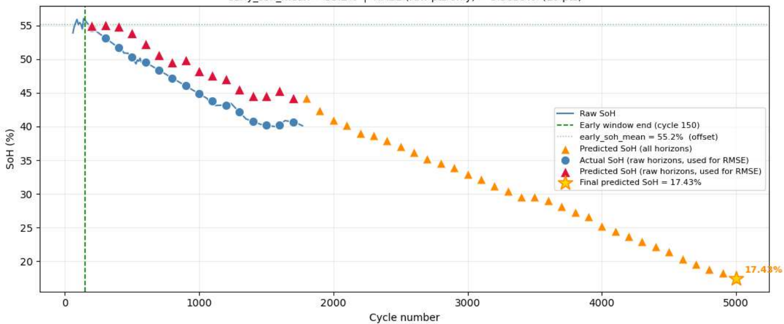
Cell 4 — Raw SoH vs Predictions early_soh_mean = 55.2% | RMSE (raw pts only) = 3.3839% (16 pts)
