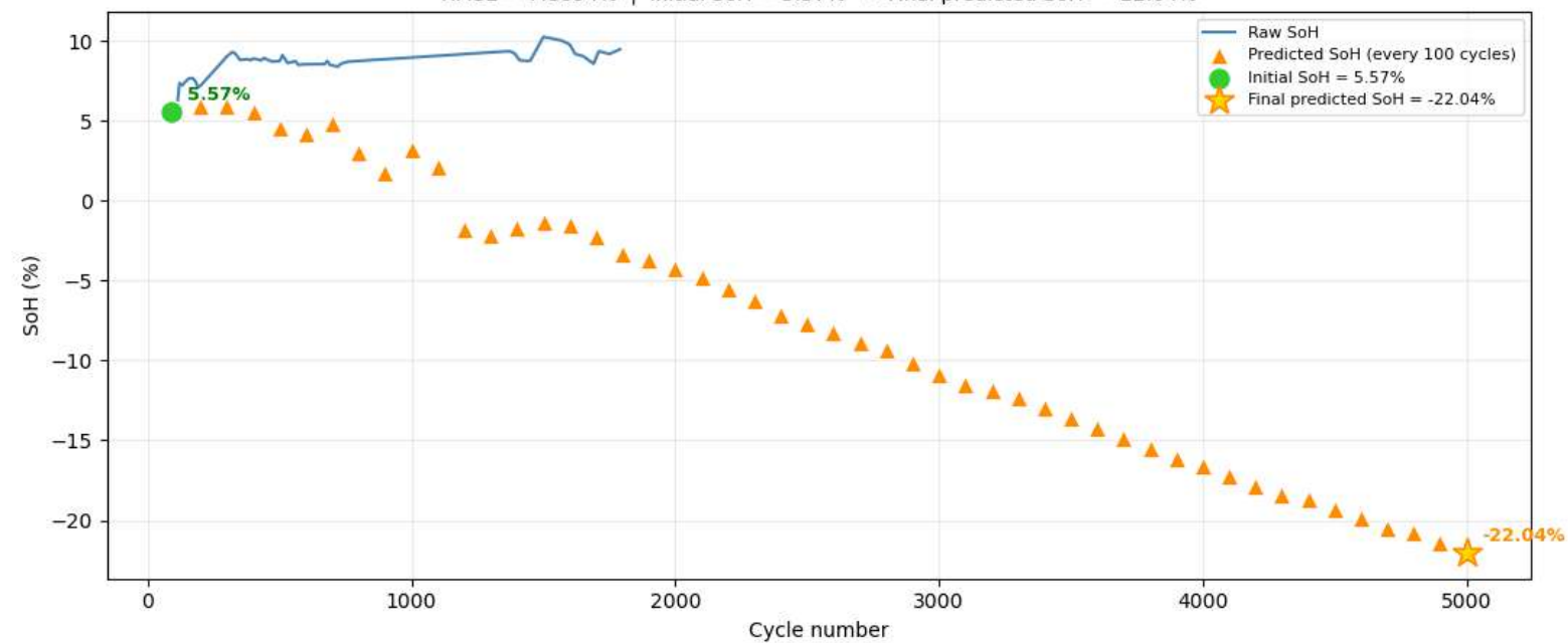
Cell 28 — Raw SoH vs Predictions RMSE = 7.8694% | Initial SoH = 5.57% → Final predicted SoH = -22.04%
