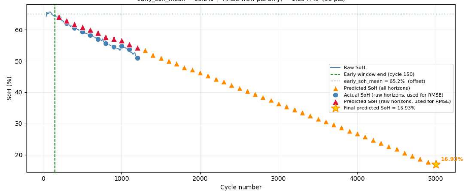
Cell 19 — Raw SoH vs Predictions early_soh_mean = 65.2% | RMSE (raw pts only) = 1.8947% (11 pts)
