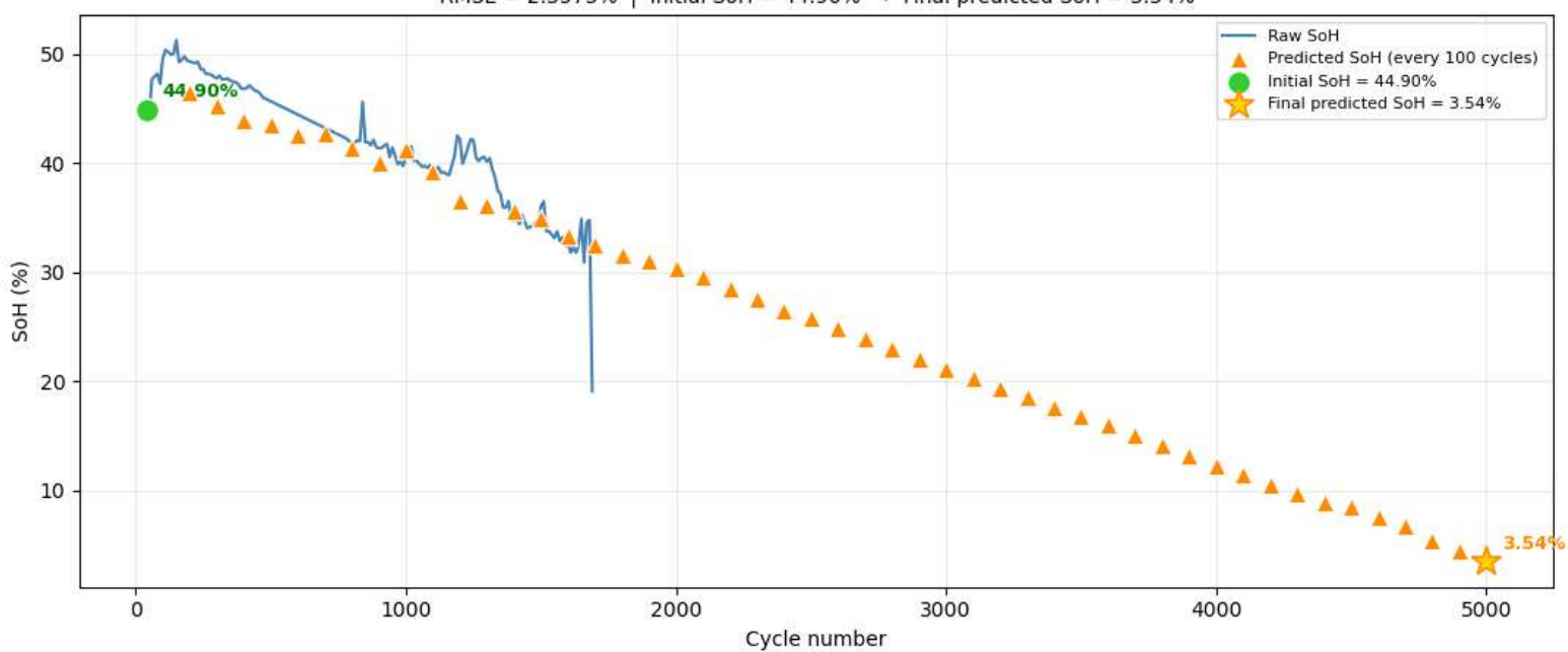
Cell 17 — Raw SoH vs Predictions RMSE = 2.3575% | Initial SoH = 44.90% → Final predicted SoH = 3.54%
