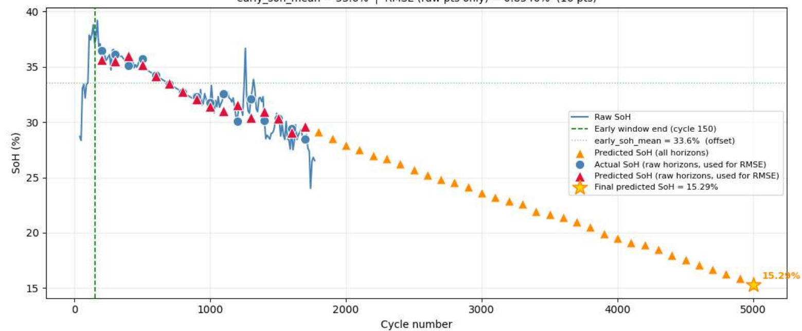
Cell 13 — Raw SoH vs Predictions early_soh_mean = 33.6% | RMSE (raw pts only) = 0.8546% (16 pts)
