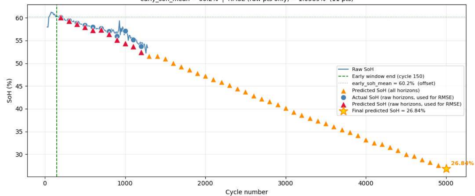
Cell 11 — Raw SoH vs Predictions early_soh_mean = 60.2% | RMSE (raw pts only) = 1.0589% (11 pts)
