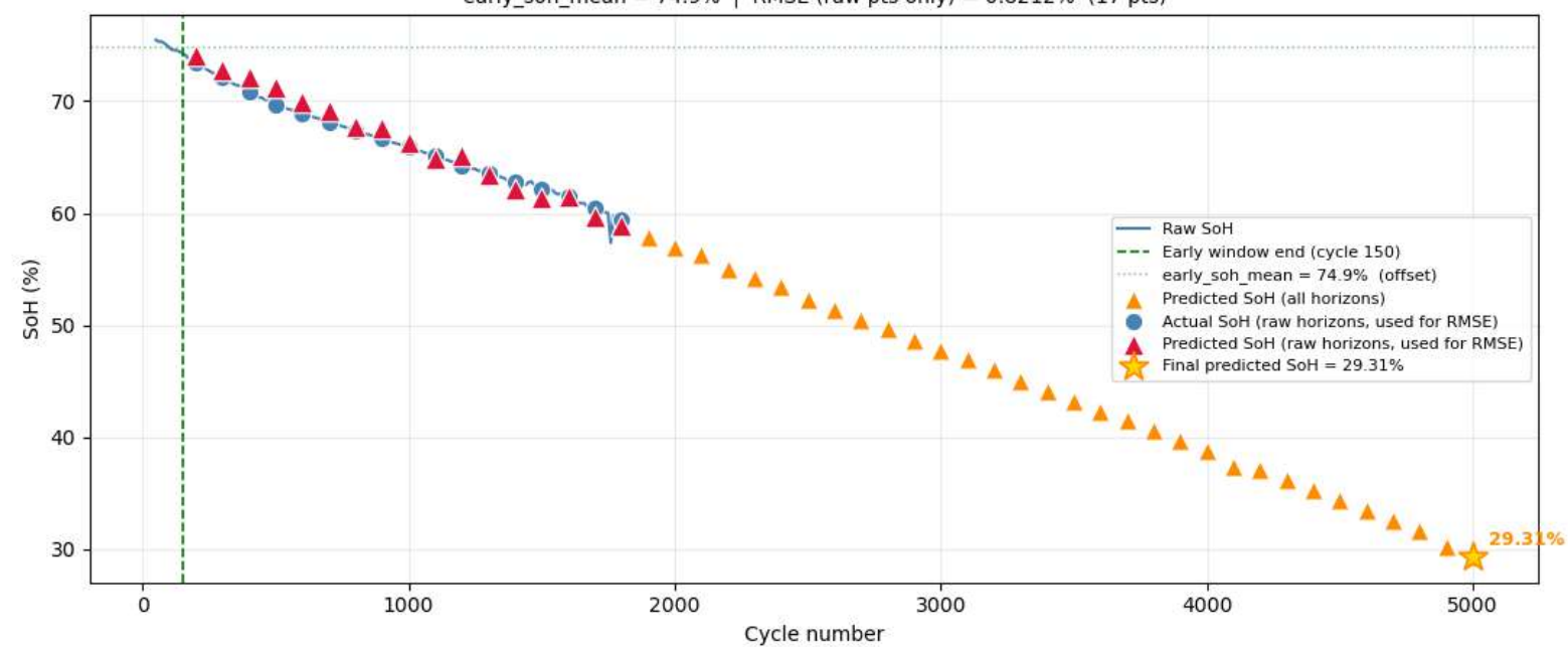
Cell 30 — Raw SoH vs Predictions early_soh_mean = 74.9% | RMSE (raw pts only) = 0.8212% (17 pts)
