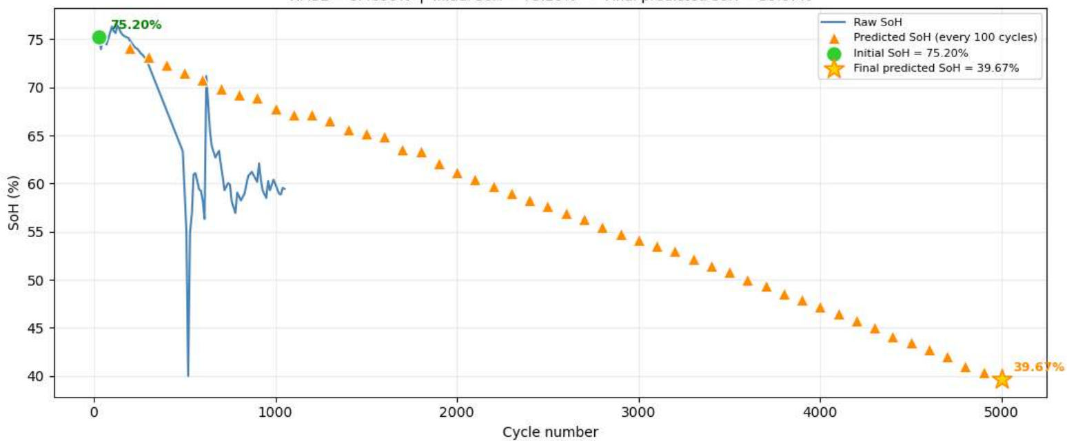
Cell 5 — Raw SoH vs Predictions RMSE = 8.4690% | Initial SoH = 75.20% → Final predicted SoH = 39.67%
