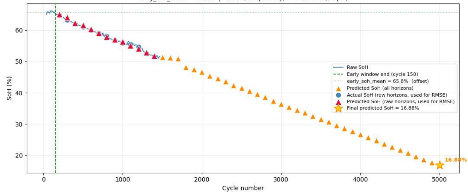
Cell 24 — Raw SoH vs Predictions early_soh_mean = 65.8% | RMSE (raw pts only) = 0.3781% (13 pts)
