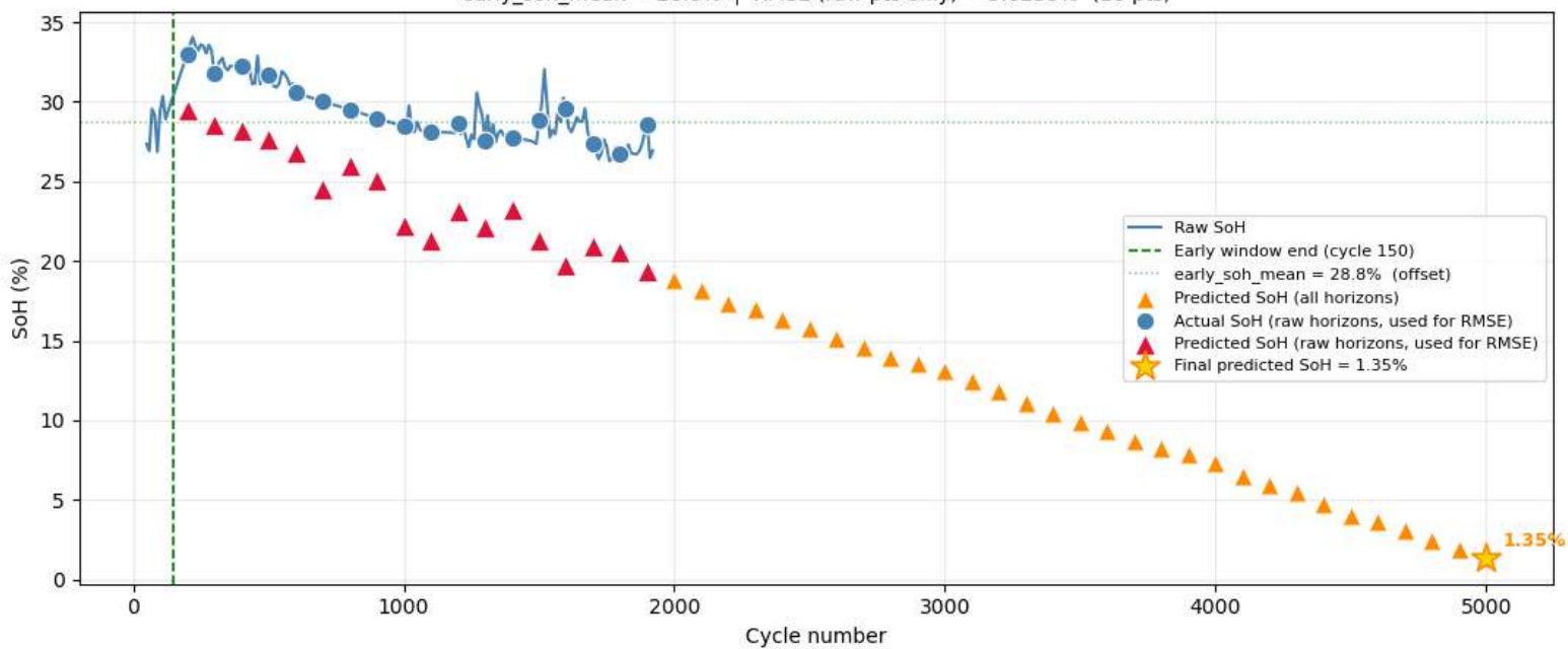
Cell 21 — Raw SoH vs Predictions early_soh_mean = 28.8% | RMSE (raw pts only) = 5.8253% (18 pts)
