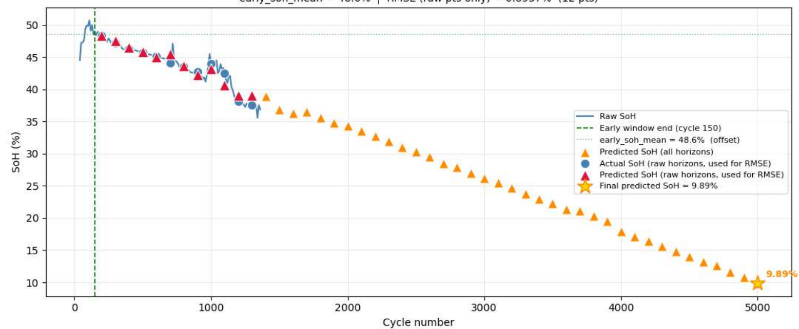
Cell 8 — Raw SoH vs Predictions early_soh_mean = 48.6% | RMSE (raw pts only) = 0.8957% (12 pts)
