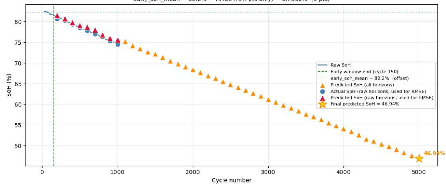
Cell 10 — Raw SoH vs Predictions early_soh_mean = 82.2% | RMSE (raw pts only) = 0.7560% (9 pts)
