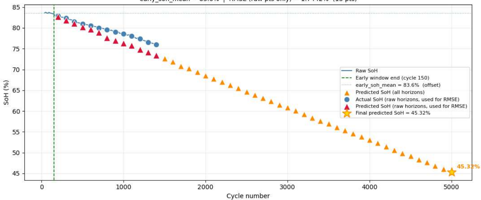
Cell 25 — Raw SoH vs Predictions early_soh_mean = 83.6% | RMSE (raw pts only) = 1.7442% (13 pts)
