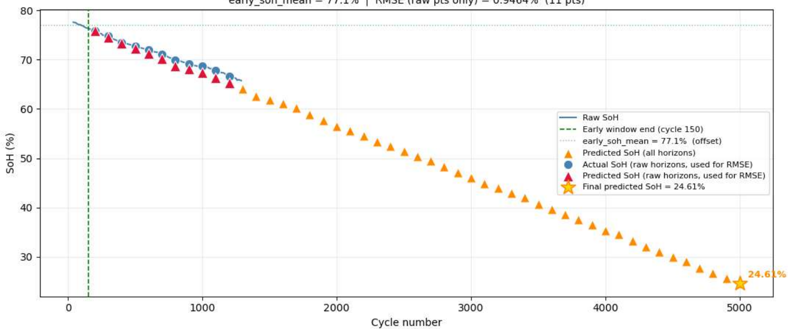
Cell 20 — Raw SoH vs Predictions early_soh_mean = 77.1% | RMSE (raw pts only) = 0.9464% (11 pts)
