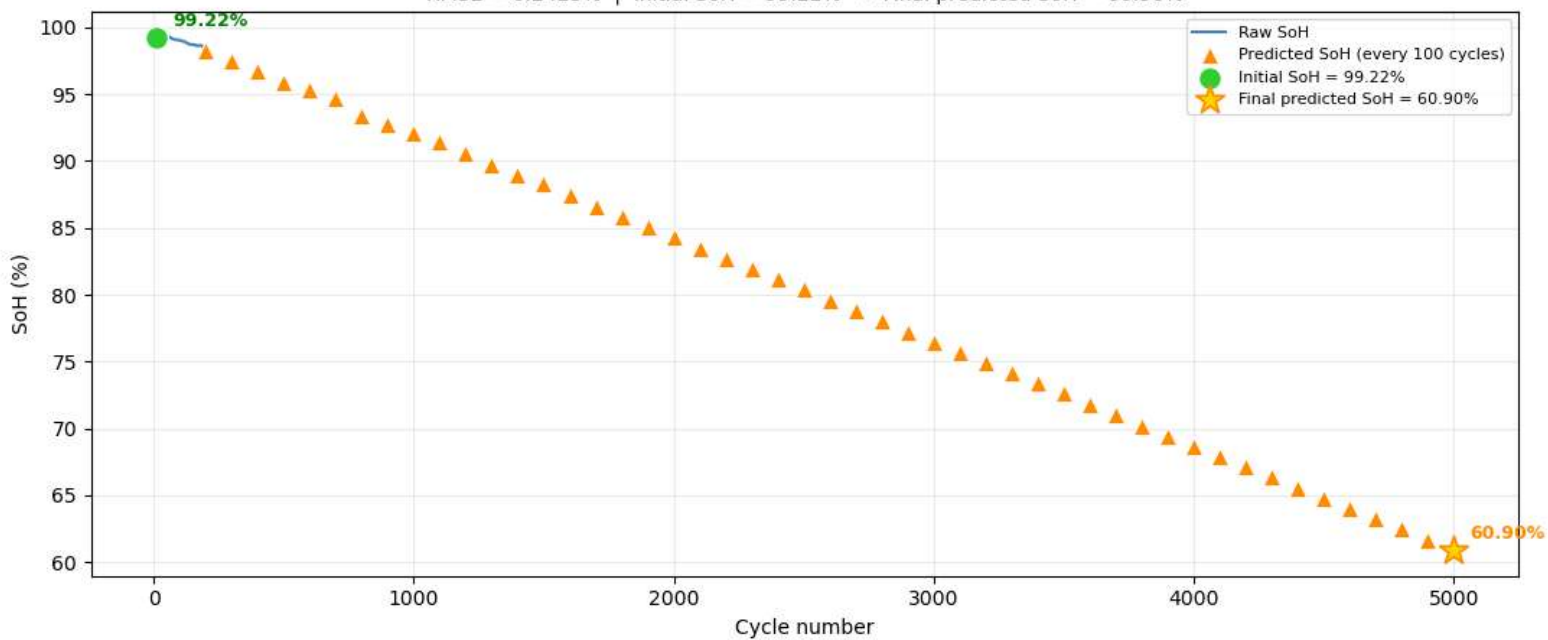
Cell 2 — Raw SoH vs Predictions RMSE = 0.2425% | Initial SoH = 99.22% → Final predicted SoH = 60.90%
