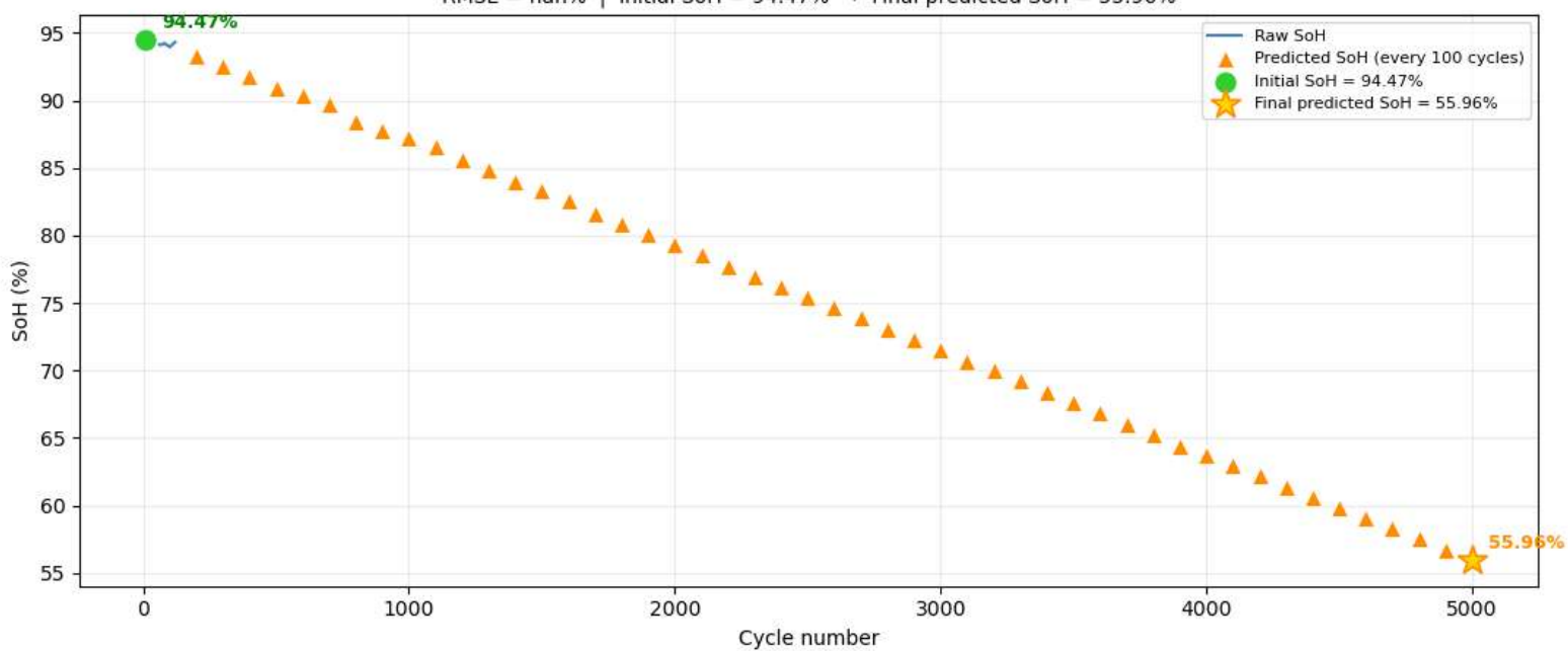
Cell 8 — Raw SoH vs Predictions RMSE = nan% | Initial SoH = 94.47% → Final predicted SoH = 55.96%
