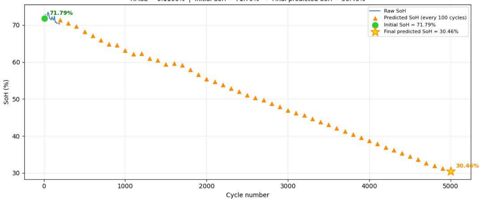
Cell 3 — Raw SoH vs Predictions RMSE = 0.1166% | Initial SoH = 71.79% → Final predicted SoH = 30.46%
