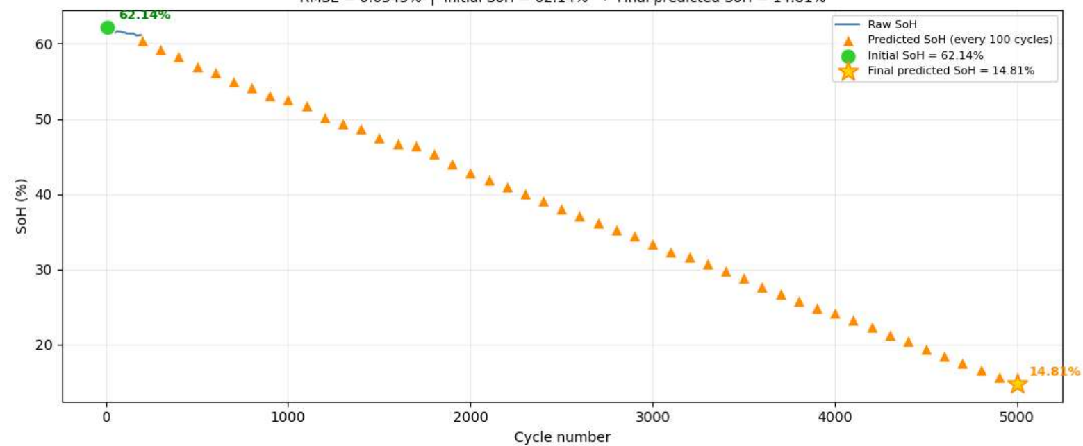
Cell 46 — Raw SoH vs Predictions RMSE = 0.6343% | Initial SoH = 62.14% → Final predicted SoH = 14.81%
