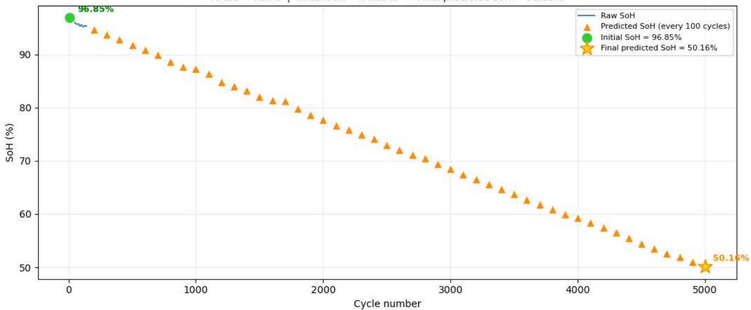
Cell 34 — Raw SoH vs Predictions RMSE = nan% | Initial SoH = 96.85% → Final predicted SoH = 50.16%
