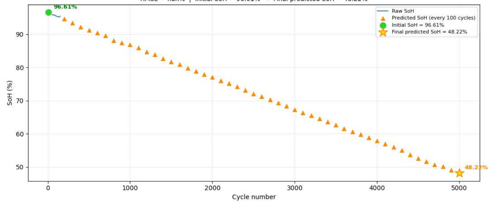
Cell 49 — Raw SoH vs Predictions RMSE = nan% | Initial SoH = 96.61% → Final predicted SoH = 48.22%
