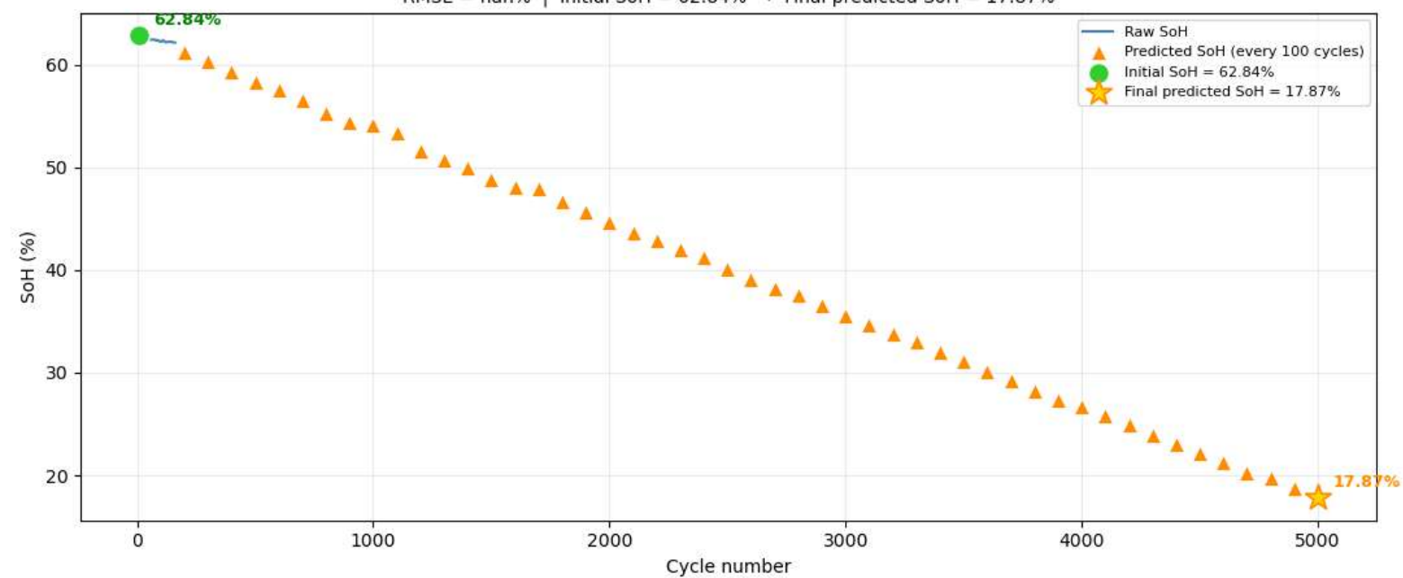
Cell 25 — Raw SoH vs Predictions RMSE = nan% | Initial SoH = 62.84% → Final predicted SoH = 17.87%
