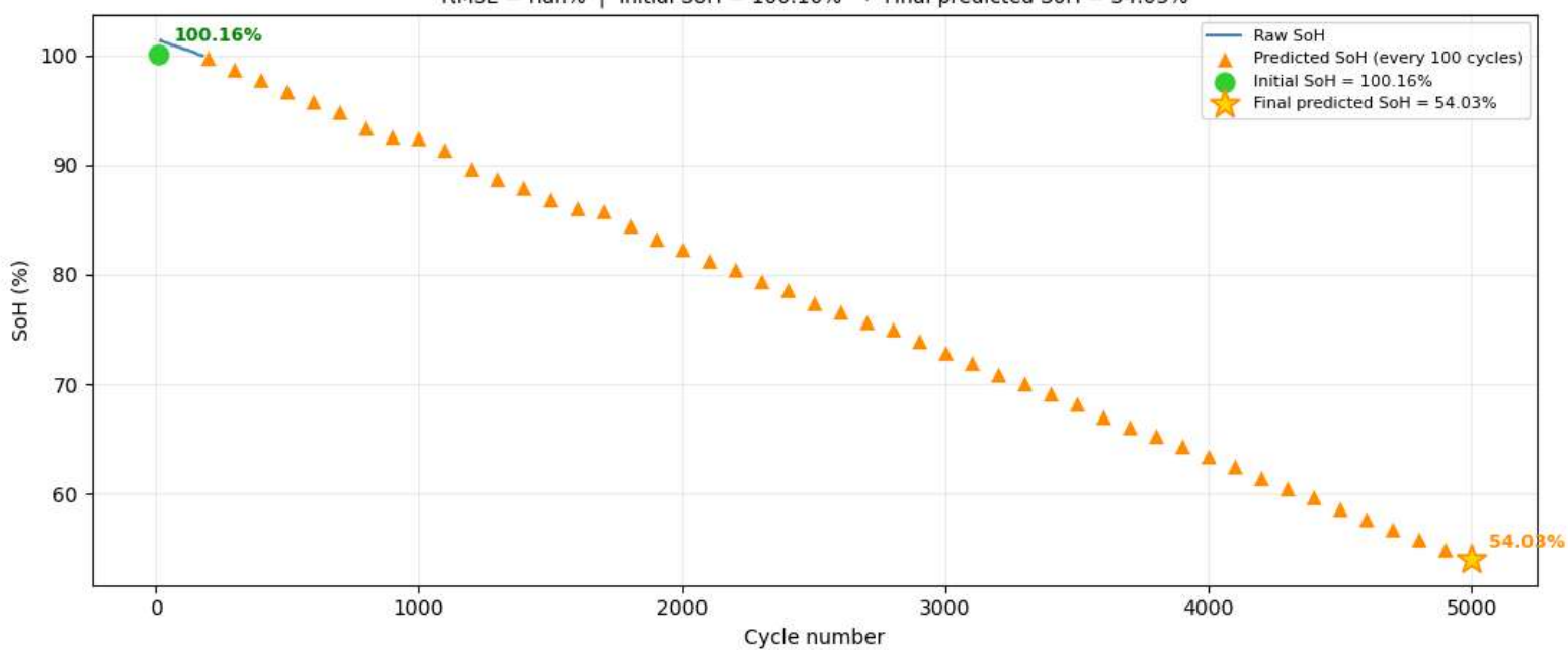
Cell 74 — Raw SoH vs Predictions RMSE = nan% | Initial SoH = 100.16% → Final predicted SoH = 54.03%
