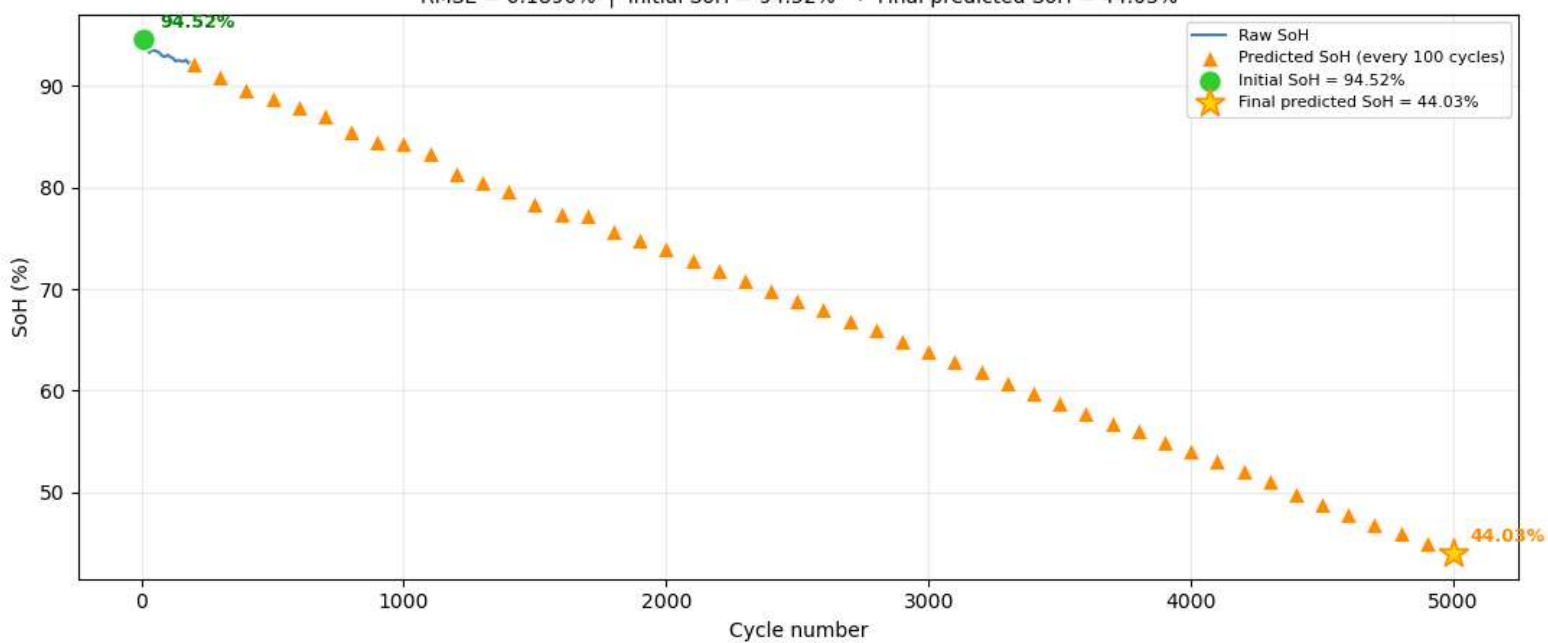
Cell 90 — Raw SoH vs Predictions RMSE = 0.1890% | Initial SoH = 94.52% → Final predicted SoH = 44.03%
