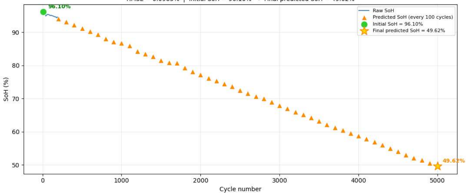
Cell 32 — Raw SoH vs Predictions RMSE = 0.0983% | Initial SoH = 96.10% → Final predicted SoH = 49.62%
