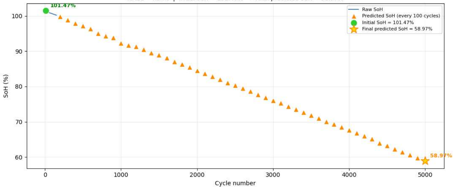
Cell 3 — Raw SoH vs Predictions RMSE = nan% | Initial SoH = 101.47% → Final predicted SoH = 58.97%
