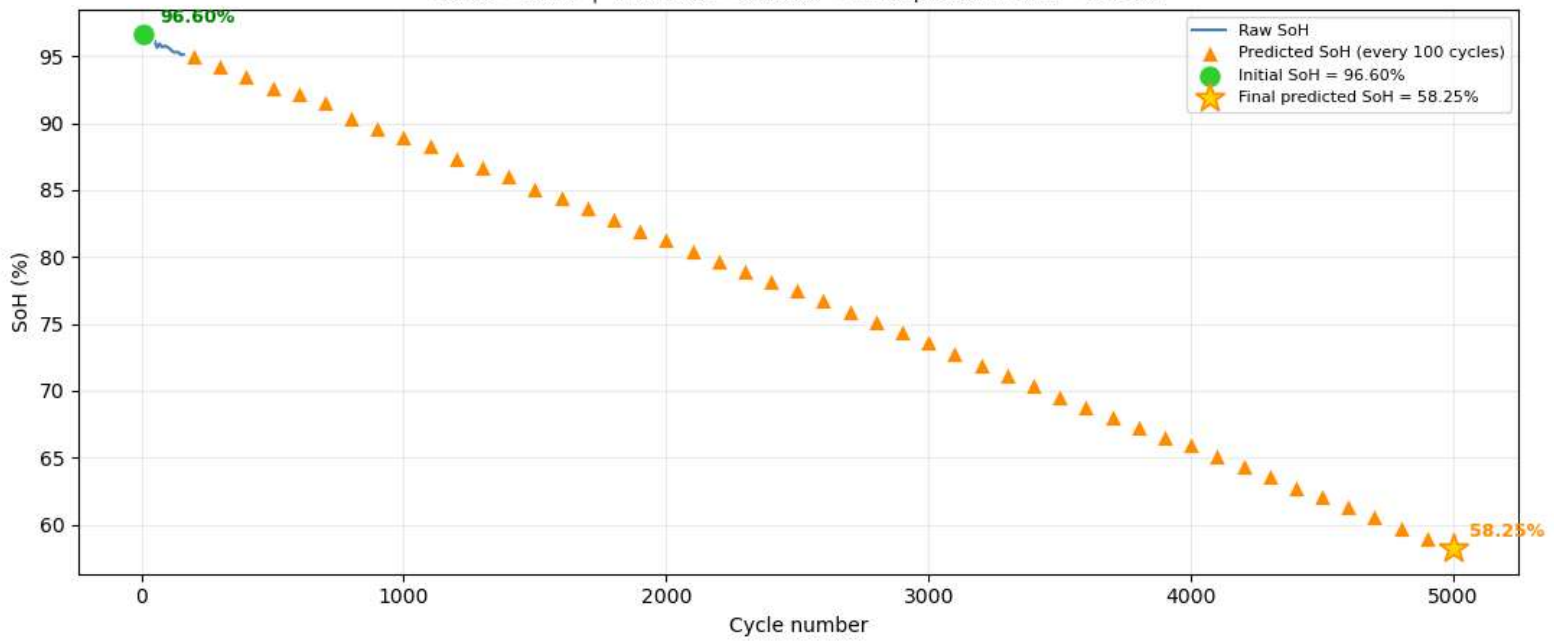
Cell 2 — Raw SoH vs Predictions RMSE = nan% | Initial SoH = 96.60% → Final predicted SoH = 58.25%
