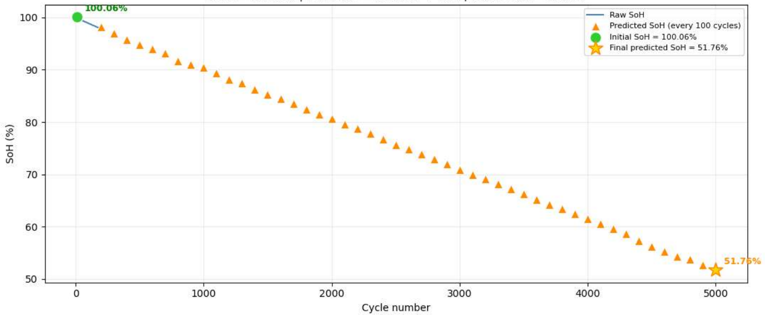
Cell 28 — Raw SoH vs Predictions RMSE = 0.3210% | Initial SoH = 100.06% → Final predicted SoH = 51.76%
