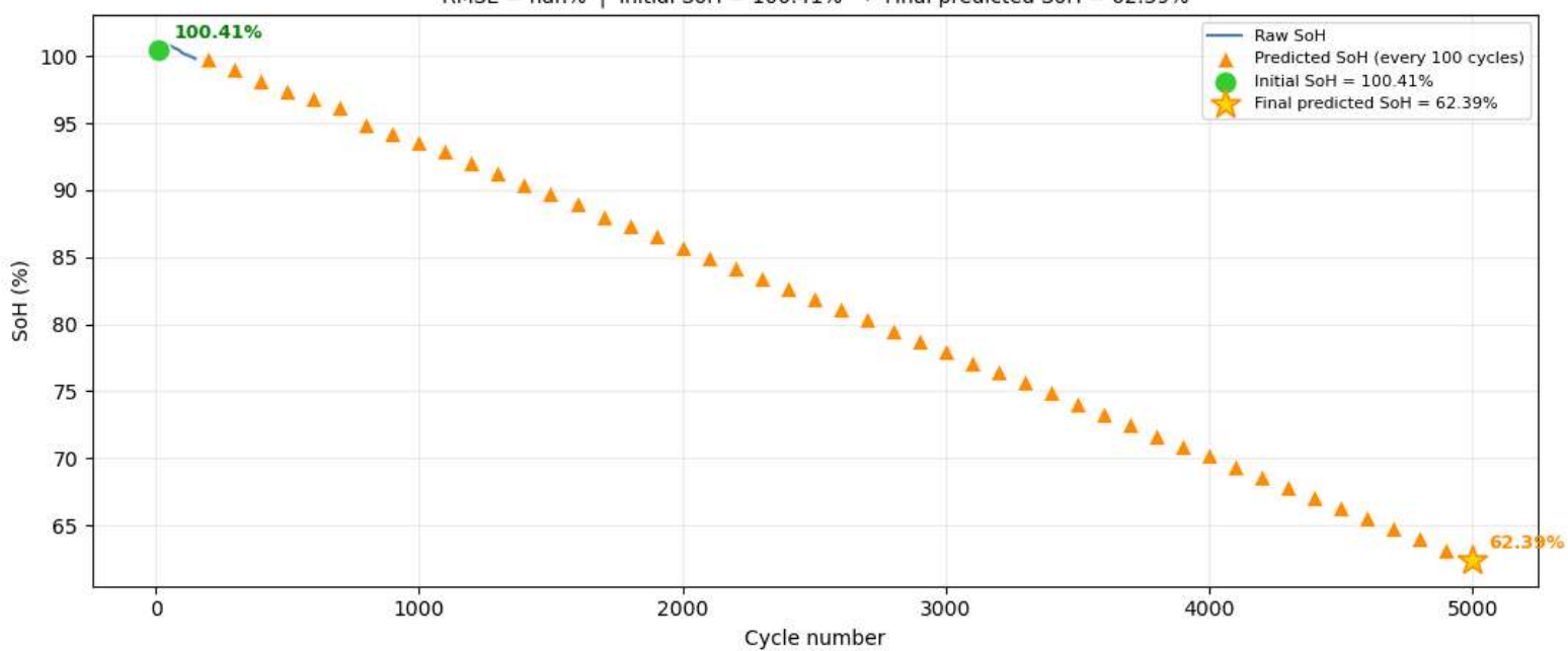
Cell 78 — Raw SoH vs Predictions RMSE = nan% | Initial SoH = 100.41% → Final predicted SoH = 62.39%
