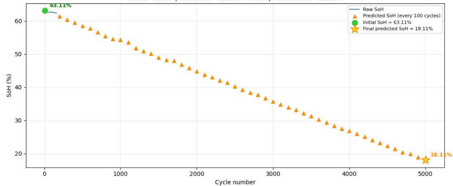
Cell 12 — Raw SoH vs Predictions RMSE = nan% | Initial SoH = 63.11% → Final predicted SoH = 18.11%
