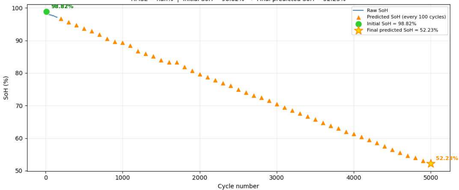
Cell 11 — Raw SoH vs Predictions RMSE = nan% | Initial SoH = 98.82% → Final predicted SoH = 52.23%
