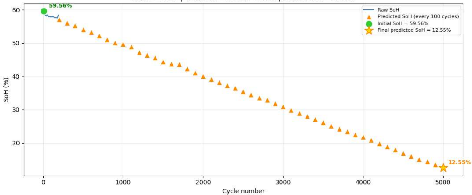
Cell 80 — Raw SoH vs Predictions RMSE = nan% | Initial SoH = 59.56% → Final predicted SoH = 12.55%
