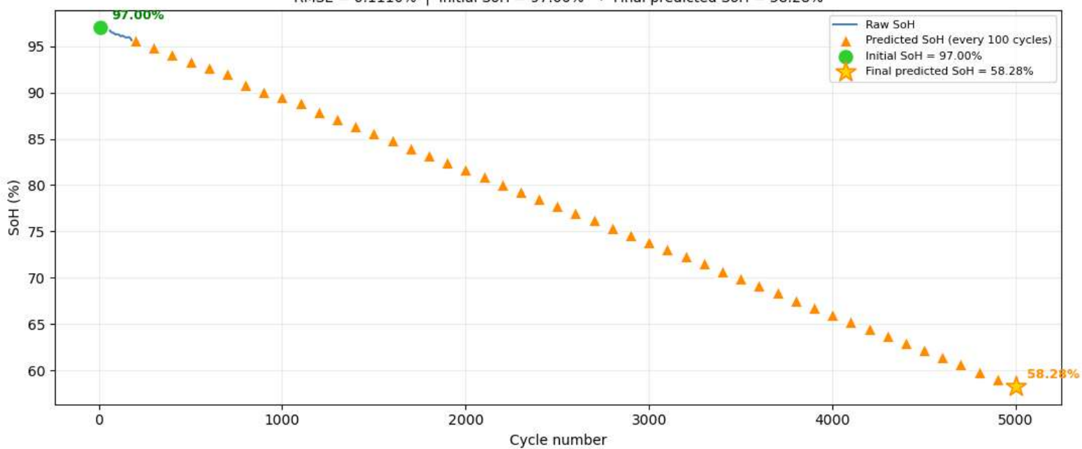
Cell 56 — Raw SoH vs Predictions RMSE = 0.1110% | Initial SoH = 97.00% → Final predicted SoH = 58.28%
