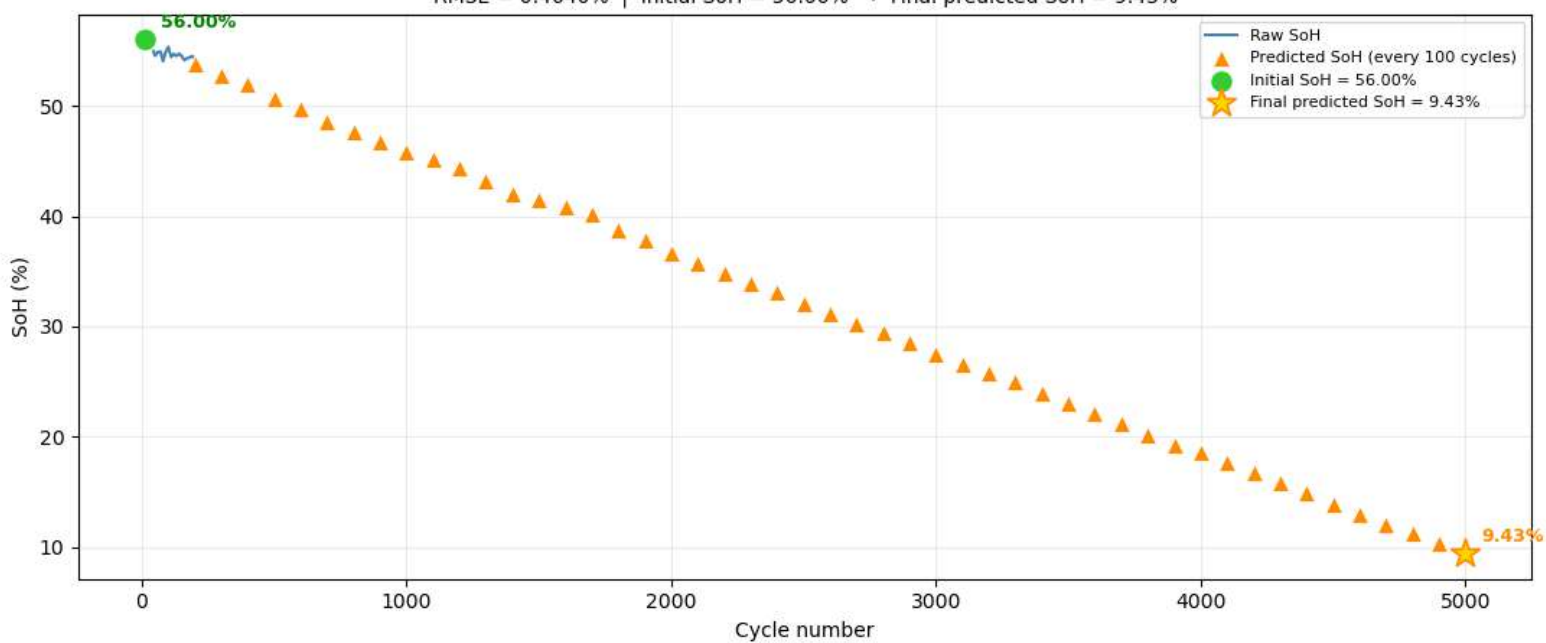
Cell 31 — Raw SoH vs Predictions RMSE = 0.4640% | Initial SoH = 56.00% → Final predicted SoH = 9.43%
