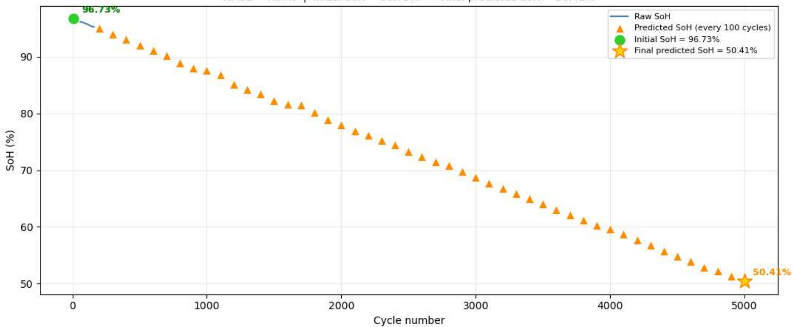
Cell 40 — Raw SoH vs Predictions RMSE = nan% | Initial SoH = 96.73% → Final predicted SoH = 50.41%
