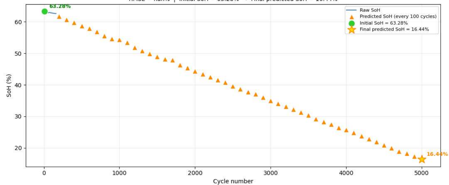
Cell 4 — Raw SoH vs Predictions RMSE = nan% | Initial SoH = 63.28% → Final predicted SoH = 16.44%
