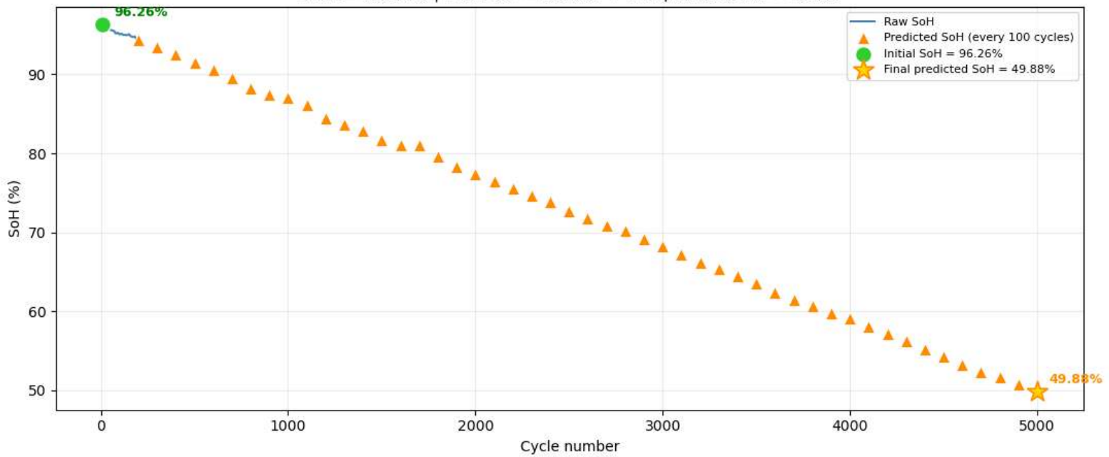
Cell 65 — Raw SoH vs Predictions RMSE = 0.0177% | Initial SoH = 96.26% → Final predicted SoH = 49.88%
