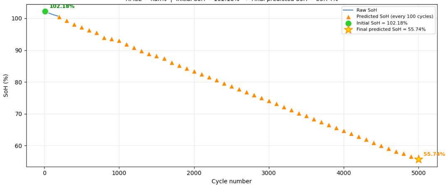
Cell 87 — Raw SoH vs Predictions RMSE = nan% | Initial SoH = 102.18% → Final predicted SoH = 55.74%
