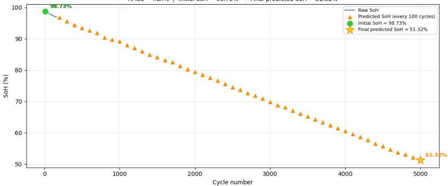
Cell 7 — Raw SoH vs Predictions RMSE = nan% | Initial SoH = 98.73% → Final predicted SoH = 51.32%
