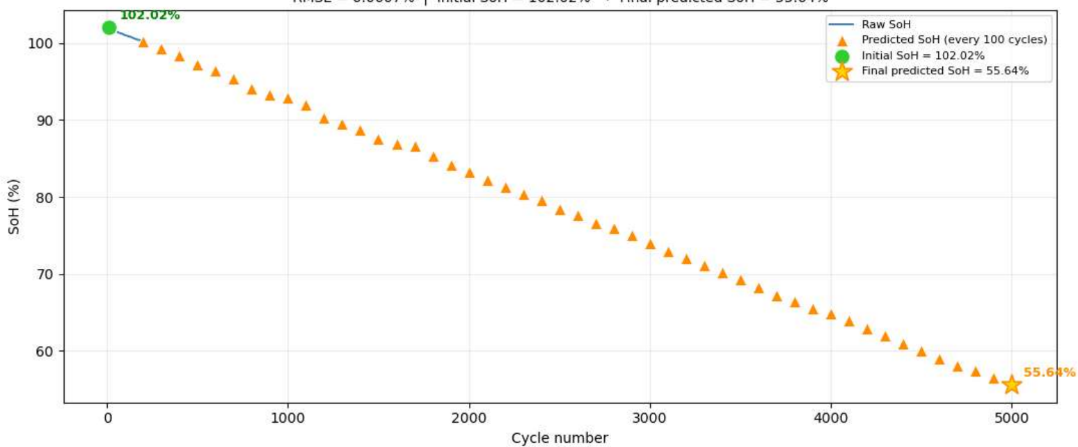
Cell 43 — Raw SoH vs Predictions RMSE = 0.0607% | Initial SoH = 102.02% → Final predicted SoH = 55.64%
