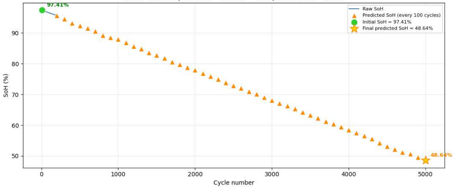
Cell 57 — Raw SoH vs Predictions RMSE = 0.0057% | Initial SoH = 97.41% → Final predicted SoH = 48.64%
