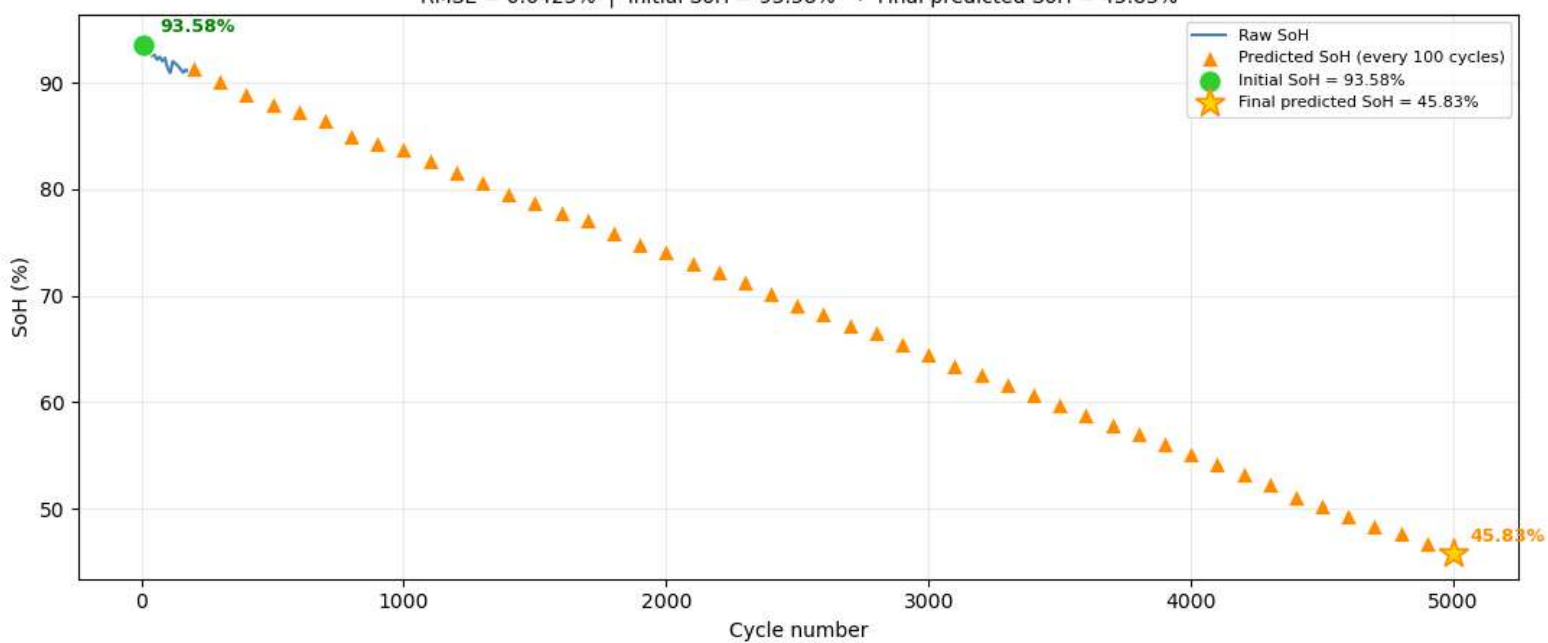
Cell 37 — Raw SoH vs Predictions RMSE = 0.6423% | Initial SoH = 93.58% → Final predicted SoH = 45.83%
