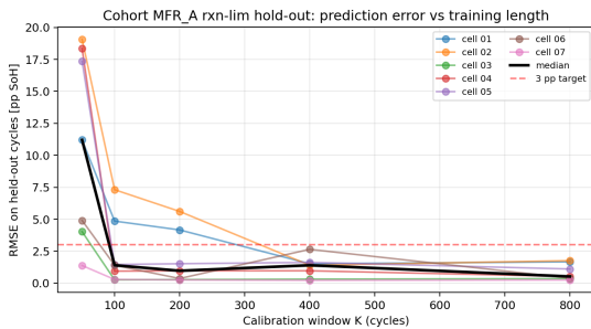
Figure 1: Held-out RMSE vs. training window K ; red dashed = 3 pp SoH target.
