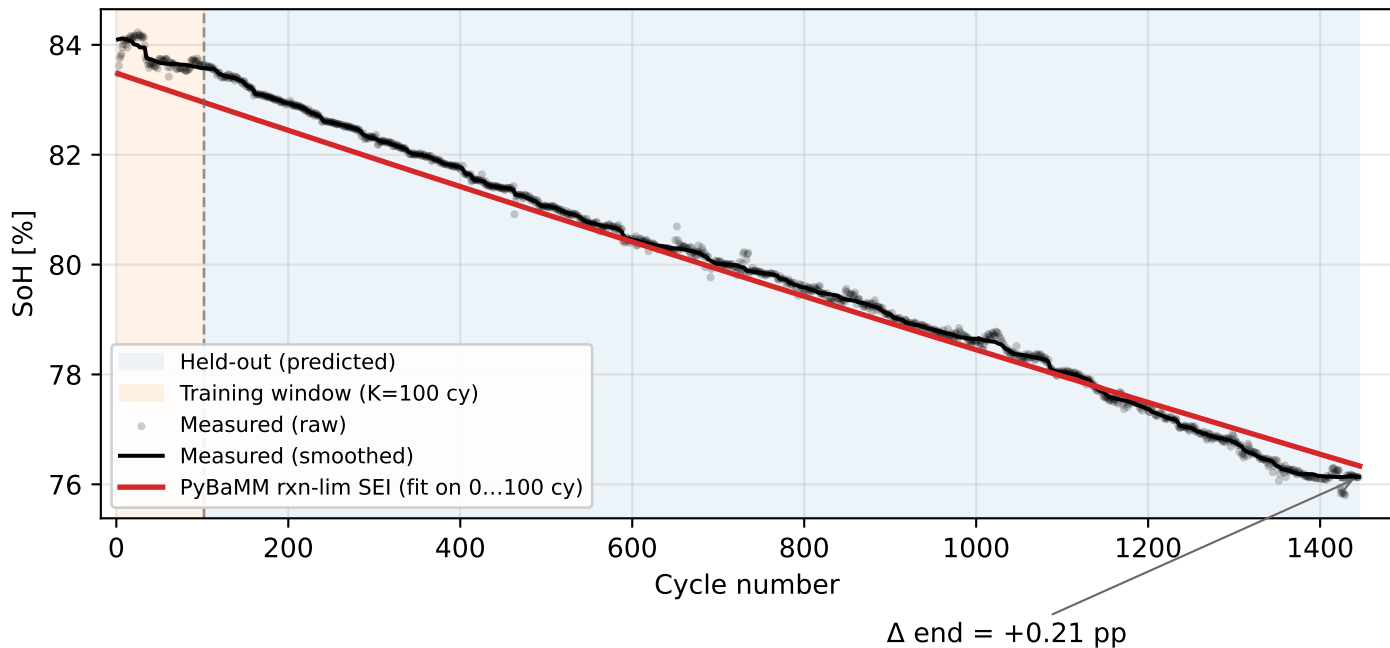
MFR_A cell 07: PyBaMM rxn-lim SEI extrapolation from 100 training cycles RMSE on held-out cycles: 0.29 pp SoH · prediction covers 1343 cycles
