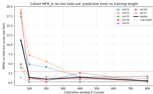
(a) Held-out RMSE vs. training window K ; red dashed = 3 pp target.
