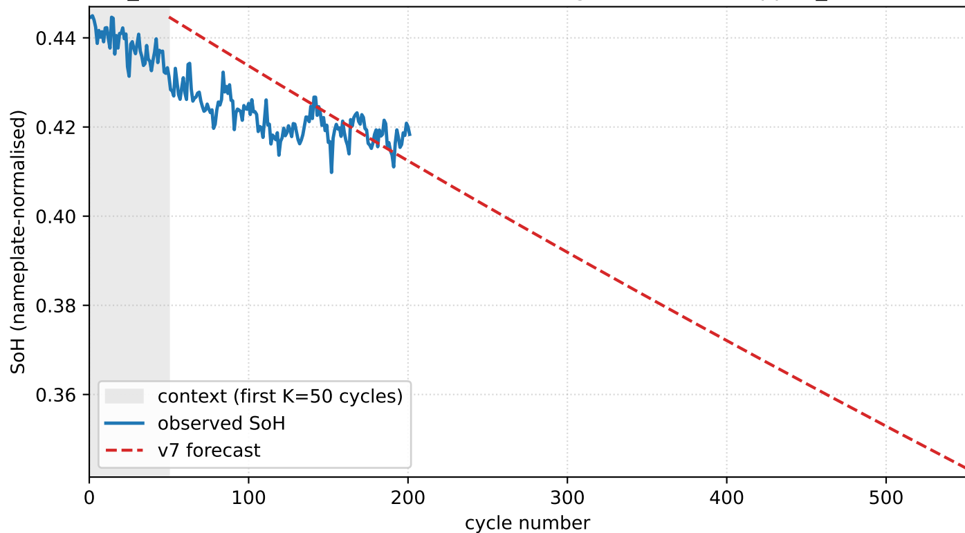
CALB_0029 — v7 held-out forecast (in-coverage RMSE = 0.95 pp, n_covered=152)
