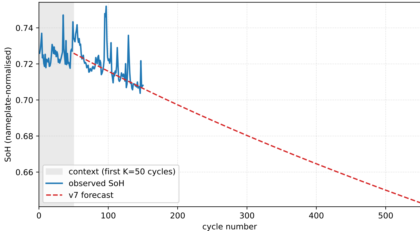
EVE_0003 — v7 held-out forecast (in-coverage RMSE = 0.83 pp, n_covered=101)
