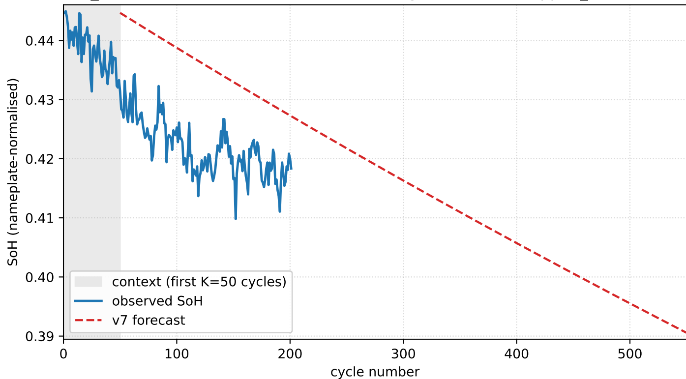
CALB_0029 — v7 held-out forecast (in-coverage RMSE = 1.46 pp, n_covered=152)
