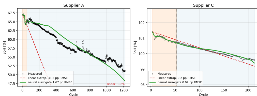
Figure 1: Best-tracking cell per supplier (ranked by peak deviation across the full held-out window). K=50 training window in orange, held-out in blue. On the deep-second-life supplier-A cell, linear-slope extrapolation (red-dashed) exits the frame while the neural surrogate (green) tracks measured across 1200+ cycles; on the light-fade supplier-C cell both methods sit under 0.2 pp.
