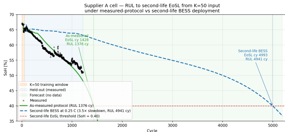
Figure 1: Neural-model RUL forecast for a deep-second-life supplier-A cell under two operating protocols. From K = 50 measured cycles (orange band), the green solid line is the as-measured-protocol extrapolation reaching EoSL at cycle 1428 (RUL 1376 cy); the blue dashed line projects the same cell under second-life BESS deployment at 0.25 C, reaching EoSL at cycle \sim 5000 (RUL 4941 cy). The neural-operator formulation retains the K=50 input budget and extends output to the full remaining-life horizon via PyBaMM-generated training trajectories.
