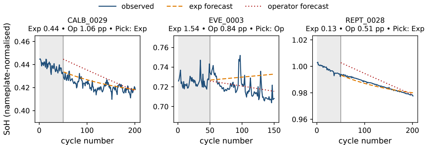
Figure 2: Forecasts evaluated against measured post-context SoH for three external cells. Grey shading denotes the K=50 context window; orange dashed and red dotted lines show exponential and neural-operator forecasts, respectively. Panels use independent y-axis ranges.
