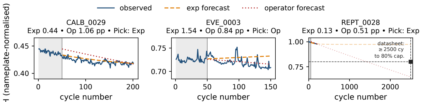
Figure 2: Forecasts evaluated against measured post-context SoH for three external cells (grey band = K=50 context; independent x/y axes). For REPT_0028, faded extensions show long-horizon projections to the datasheet cycle-life reference ( \geq 2500 cycles to 80% capacity) — not a measured continuation of the cell.
