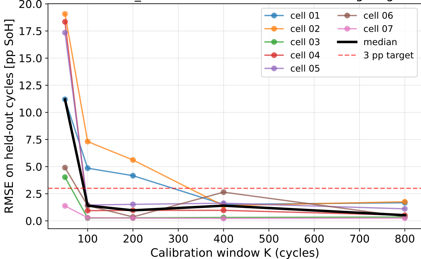
Cohort MFR_A rxn-lim hold-out: RMSE vs training length
