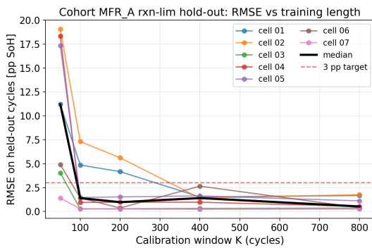
Figure 1: Held-out RMSE vs. training window K ; red dashed = 3 pp SoH target.
