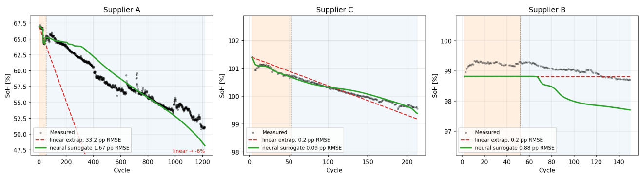
Figure 1: One representative cell per supplier, ranked by peak deviation across the full held-out window ( K=50 training in orange, held-out in blue). On the deep-second-life supplier-A cell, linear-slope extrapolation (red-dashed) exits the frame while the neural surrogate (green) tracks measured across 1200+ cycles; on the light-fade supplier-C and supplier-B cells both methods sit under 1 pp.
