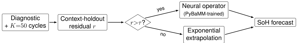
Figure 1: Adaptive selector: a context-holdout residual (exp fit on first 80% of the K=50 context, RMSE on last 20%) picks the neural operator above threshold \tau ; \tau is set on synthetic trajectories only.
