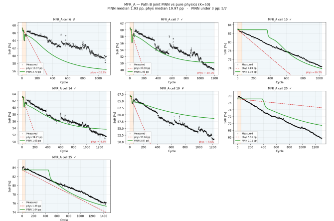
Figure 2: MFR_A trajectories (K=50). Naïve linear extrapolation exits the frame with impossible-SoH annotations; the PyBaMM-constrained PINN tracks measured.
