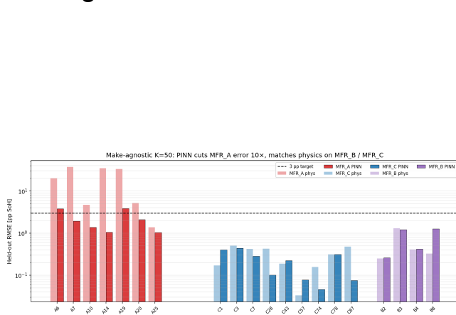
Figure 1: Per-cell held-out RMSE across 3 manufacturers (log scale). Short-window linear SEI-slope extrapolation towers above the 3 pp target on MFR_A; the PyBaMM-informed PINN is matched or below across all makes.
