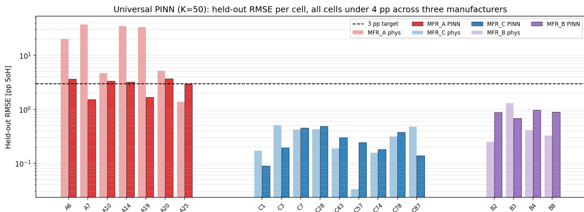
Figure 1: Held-out RMSE per cell across three LFP suppliers (log scale), from 50 training cycles. Linear-slope extrapolation towers above the 3 pp target on the deep-second-life supplier-A cohort; the neural surrogate stays under 4 pp on every cell across all three suppliers.
