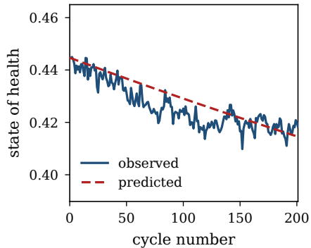
CALB_0029 (fast (EoL 292 cy))
