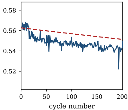
REPT_0031 (mid (212 cy pre-knee))
