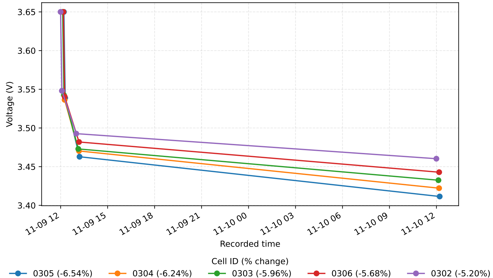
Recorded Time vs Voltage - 09 Nov 2025
