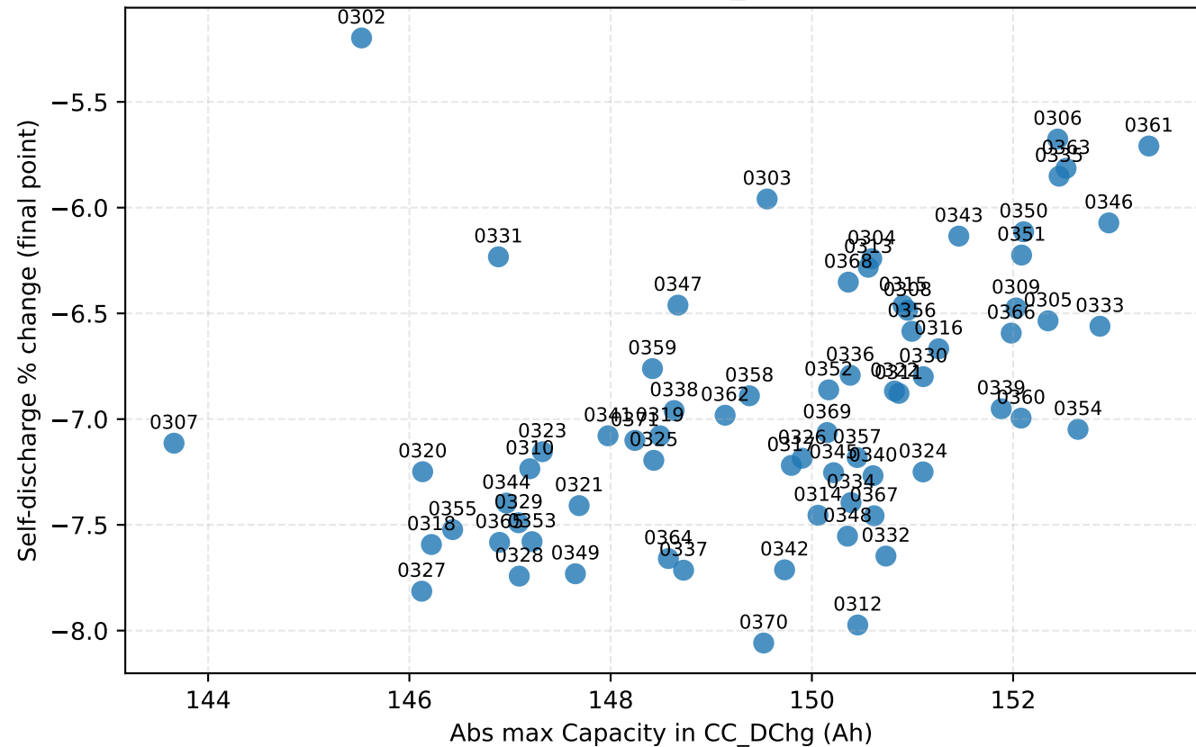
Self-Discharge % Change vs CC_DChg Capacity (RPT)
