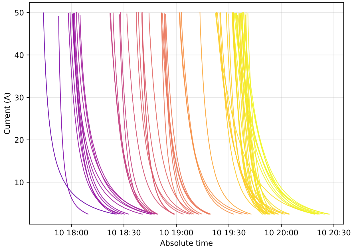
CCCV_Chg — CV current vs absolute time | 2025-11-10
