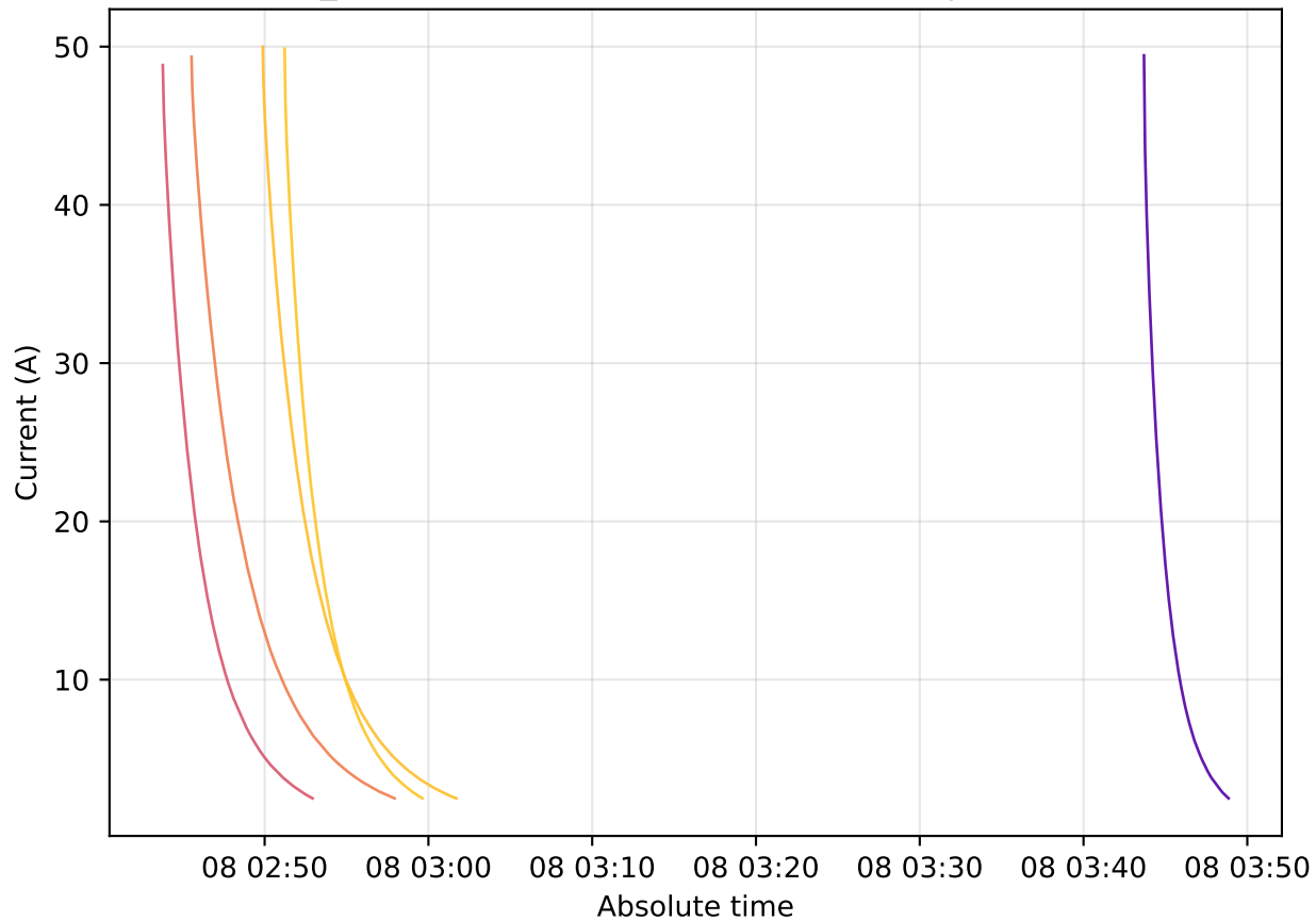
CCCV_Chg — CV current vs absolute time | 2025-11-08
