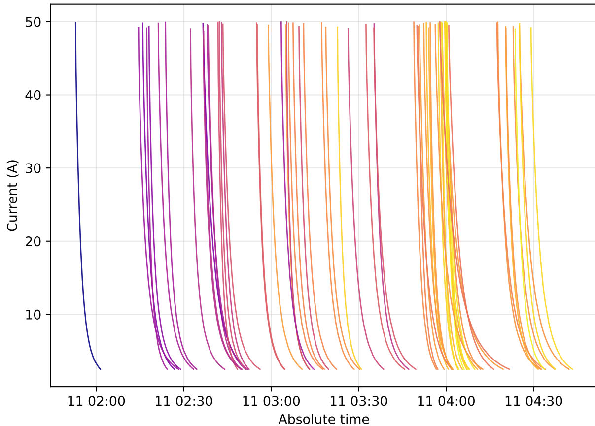
CCCV_Chg — CV current vs absolute time | 2025-11-11
