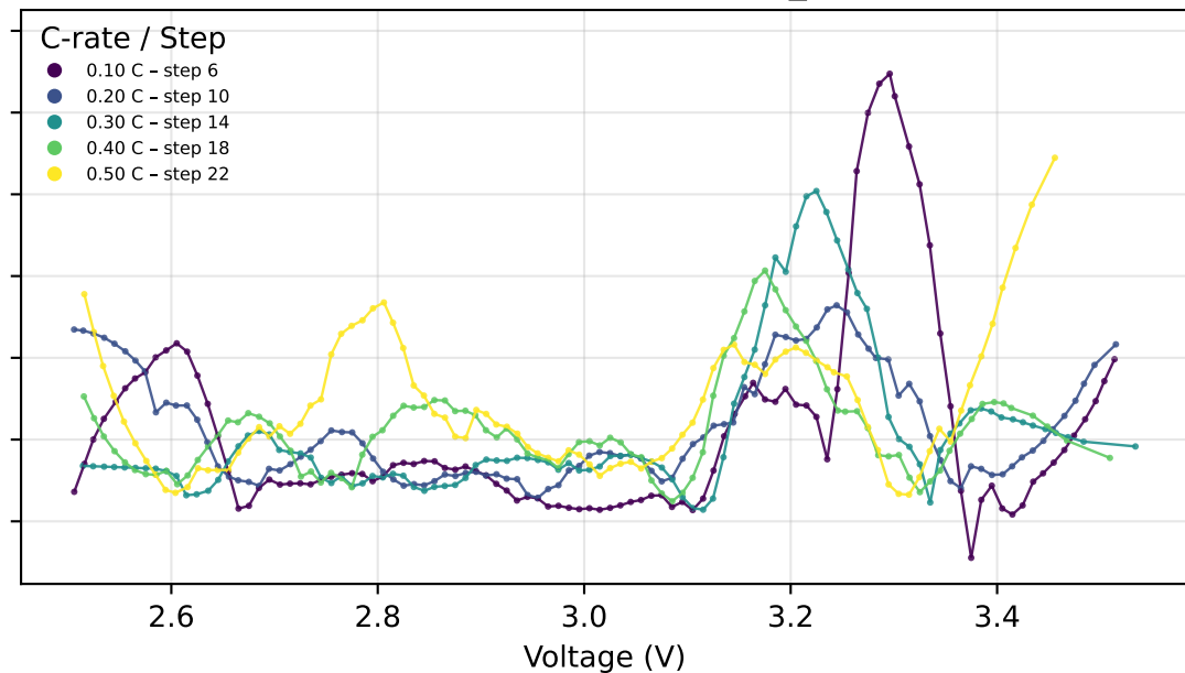
Discharge - Cycle 2 - T 1
