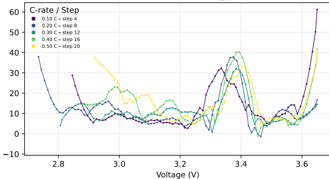
Charge - Cycle 1 - T_4
