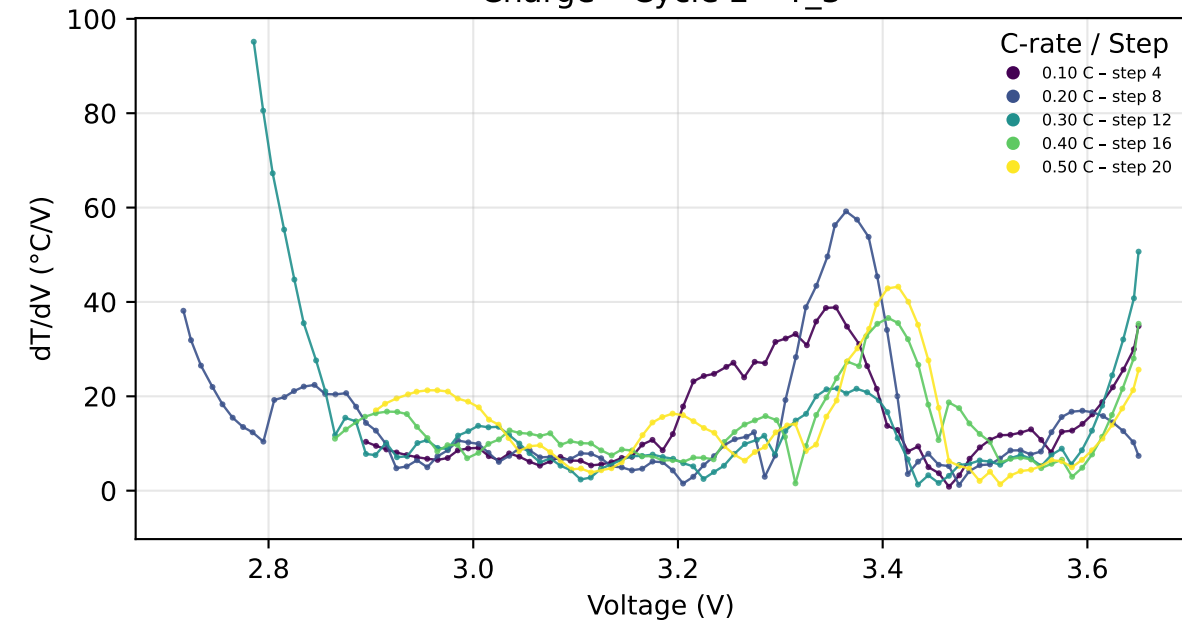
Charge - Cycle 2 - T_3
