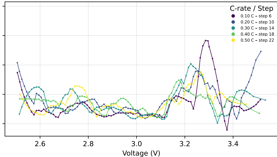
Discharge - Cycle 2 - T 4
