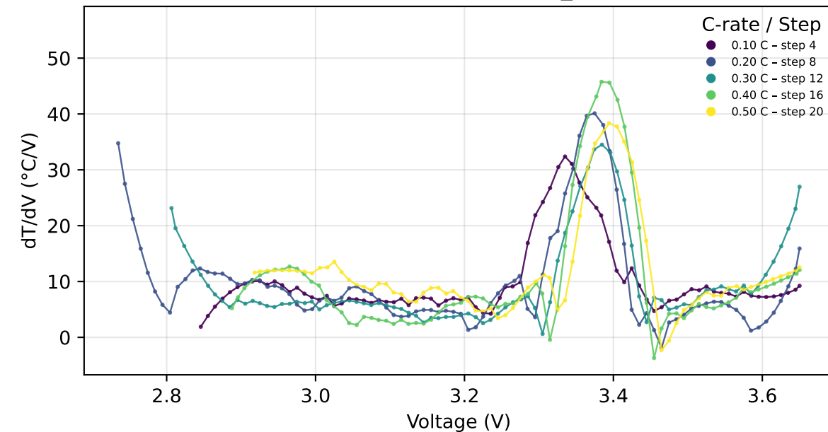
Charge - Cycle 1 - T_1
