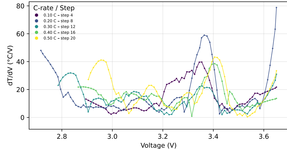
Charge - Cycle 2 - T 4
