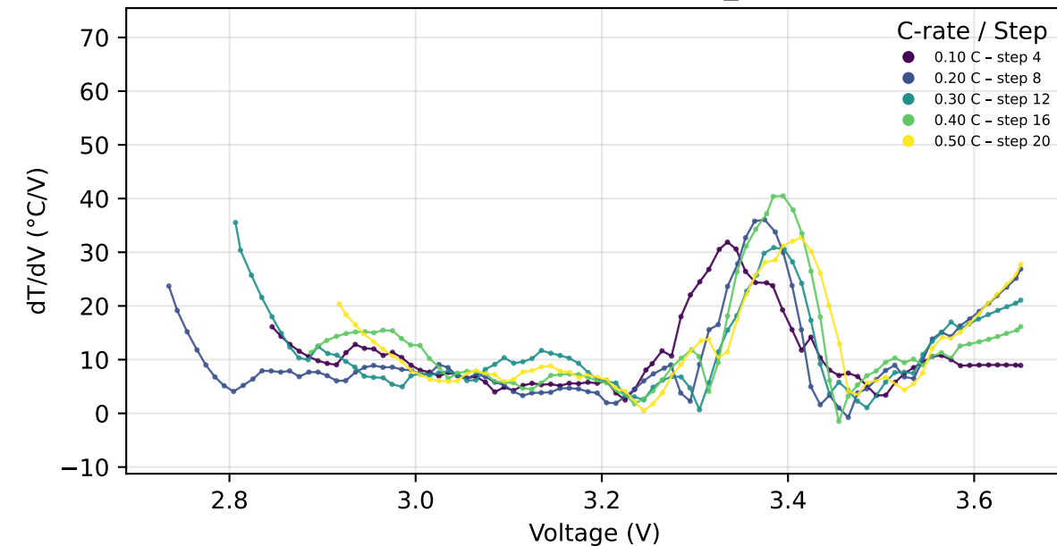
Charge - Cycle 1 - T_3
