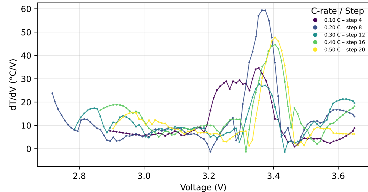
Charge - Cycle 2 - T 1
