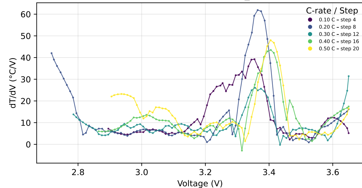
Charge - Cycle 2 - T 2
