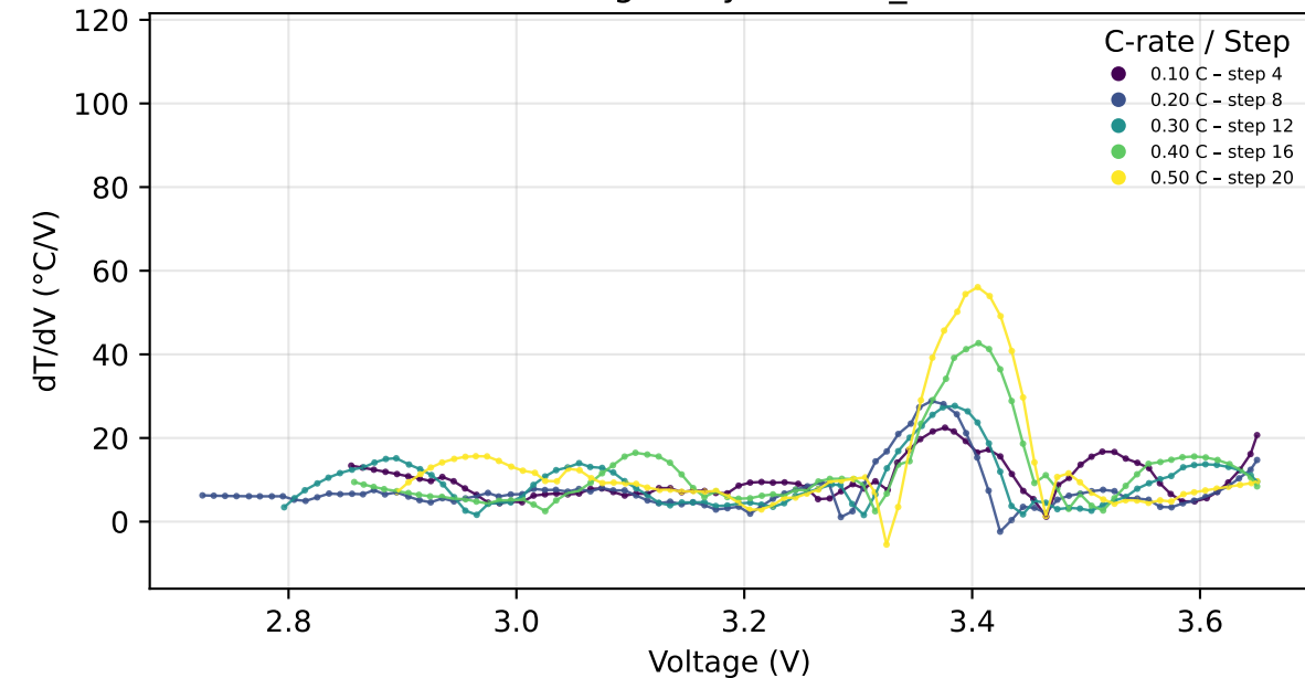
Charge - Cycle 3 - T 2
