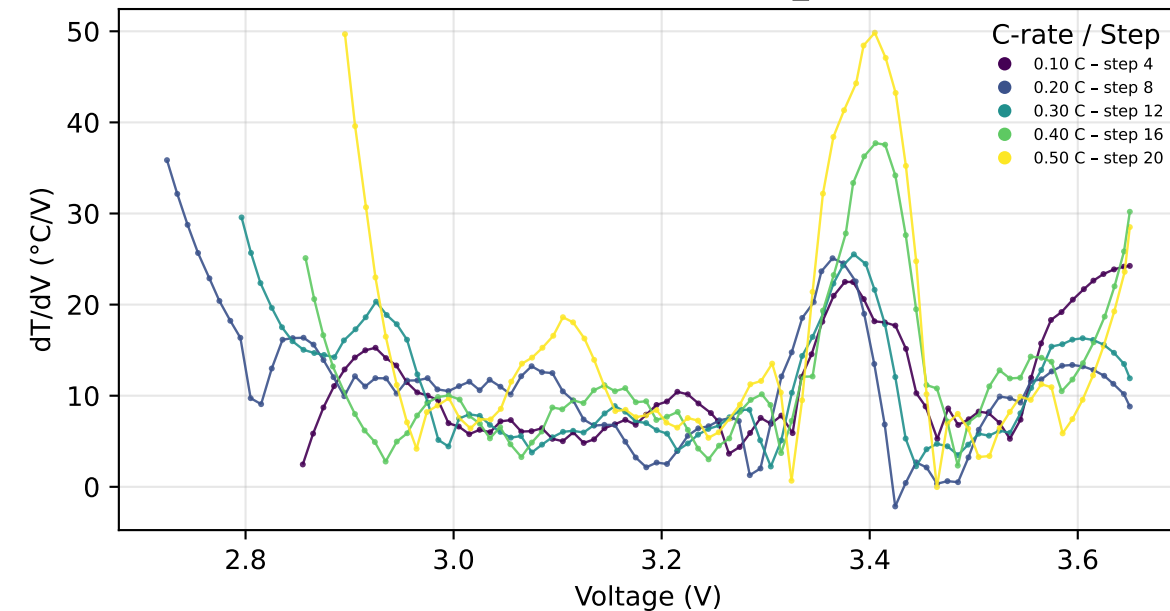
Charge - Cycle 3 - T 3
