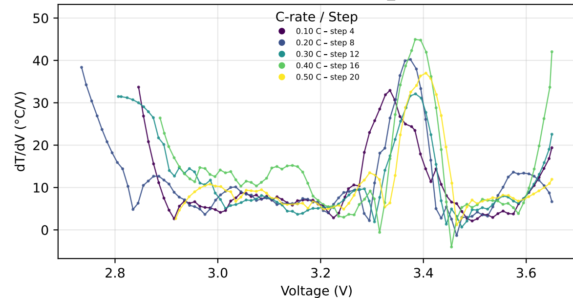
Charge - Cycle 1 - T 2
