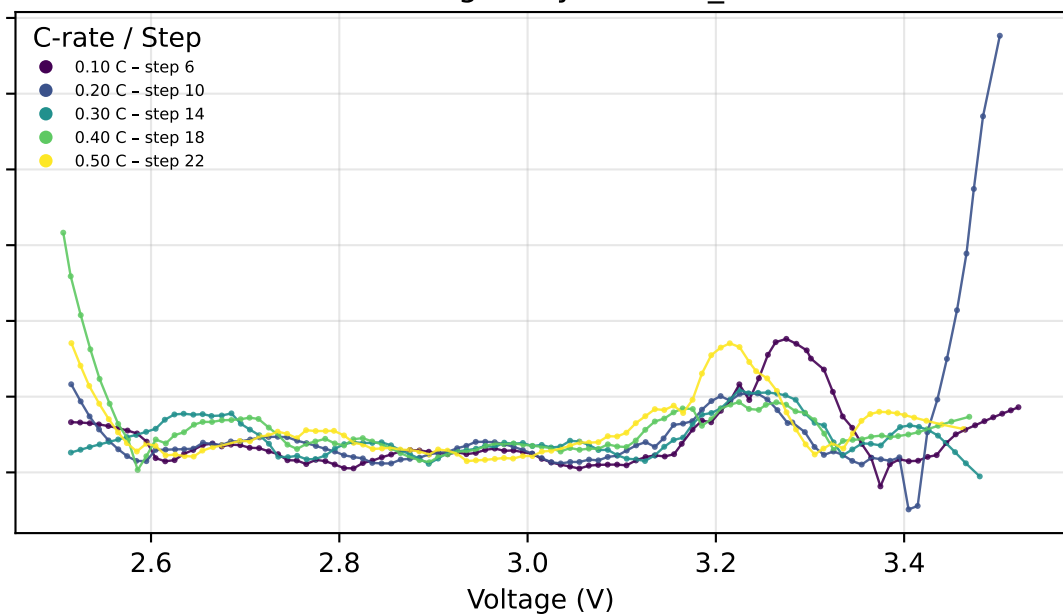
Discharge - Cycle 3 - T 2
