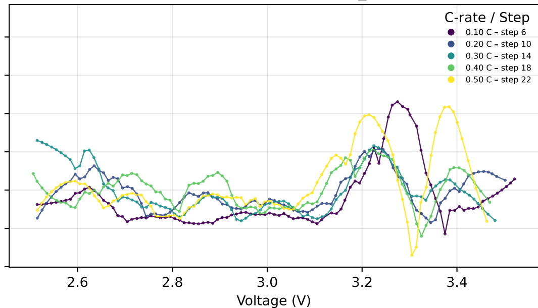
Discharge - Cycle 3 - T 1
