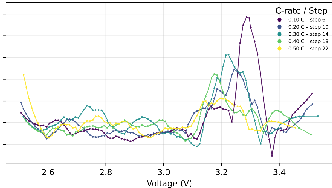
Discharge - Cycle 2 - T 2
