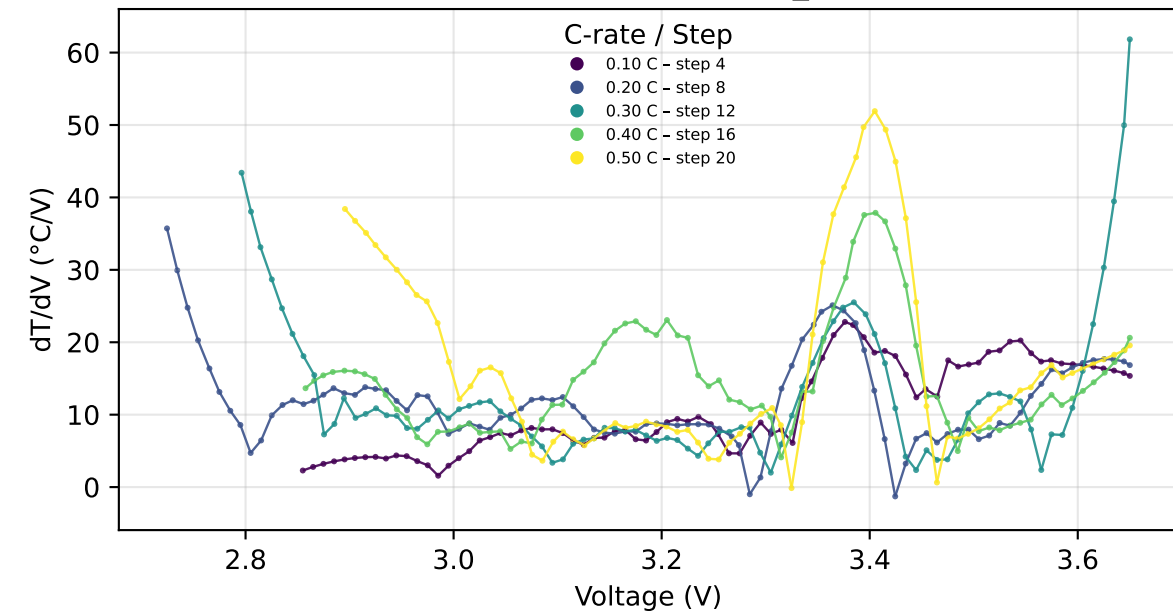
Charge - Cycle 3 - T 4
