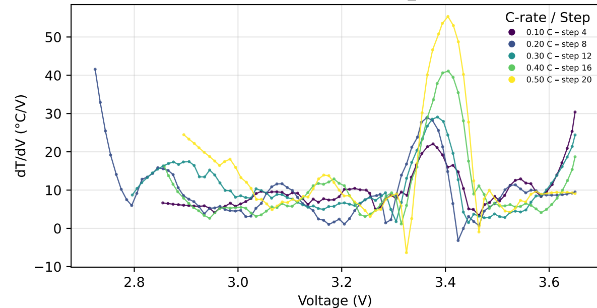
Charge - Cycle 3 - T 1
