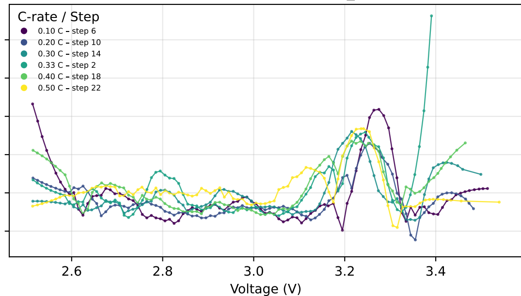
Discharge - Cycle 1 - T_1
