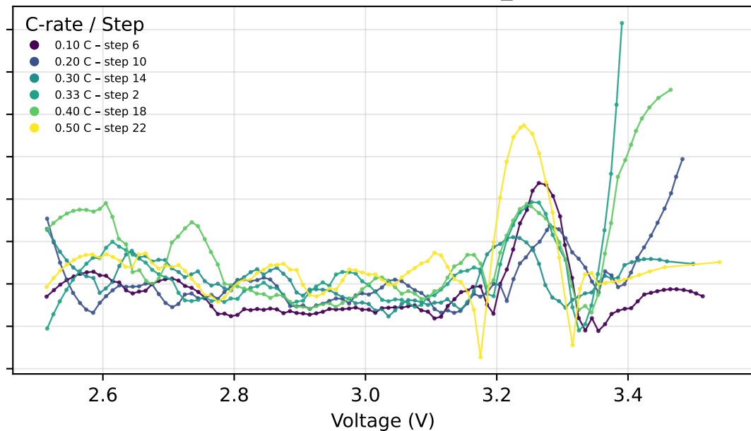
Discharge - Cycle 1 - T_3
