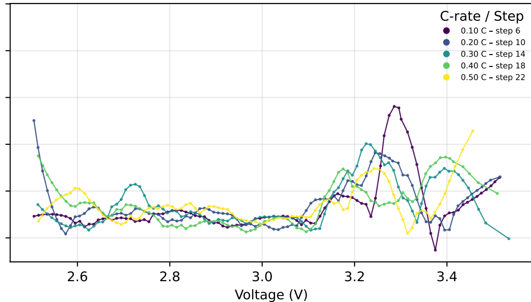
Discharge - Cycle 2 - T_3
