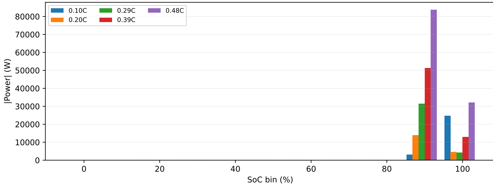
RD_RateCapability_0012 - CCCV_Chg
