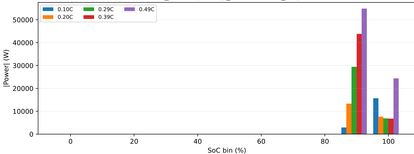
RD_RateCapability_0078 - CCCV_Chg
