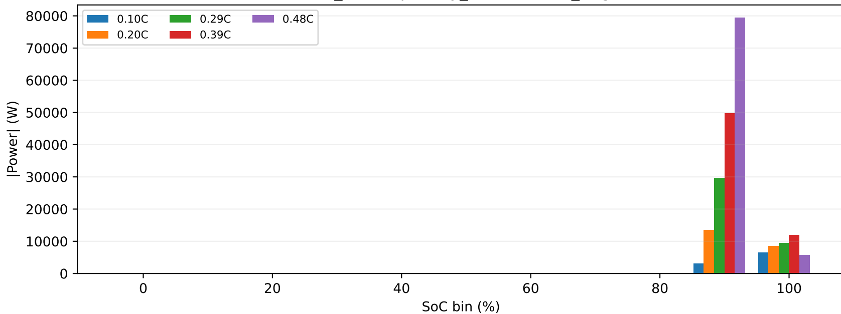
RD_RateCapability_0080 - CCCV_Chg
