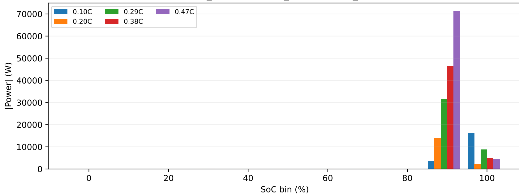
RD_RateCapability_0034 - CCCV_Chg
