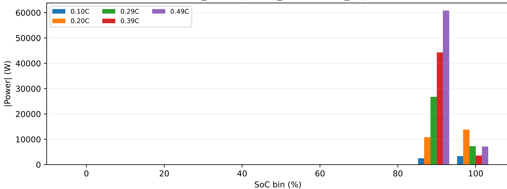
RD_RateCapability_0057 - CCCV_Chg
