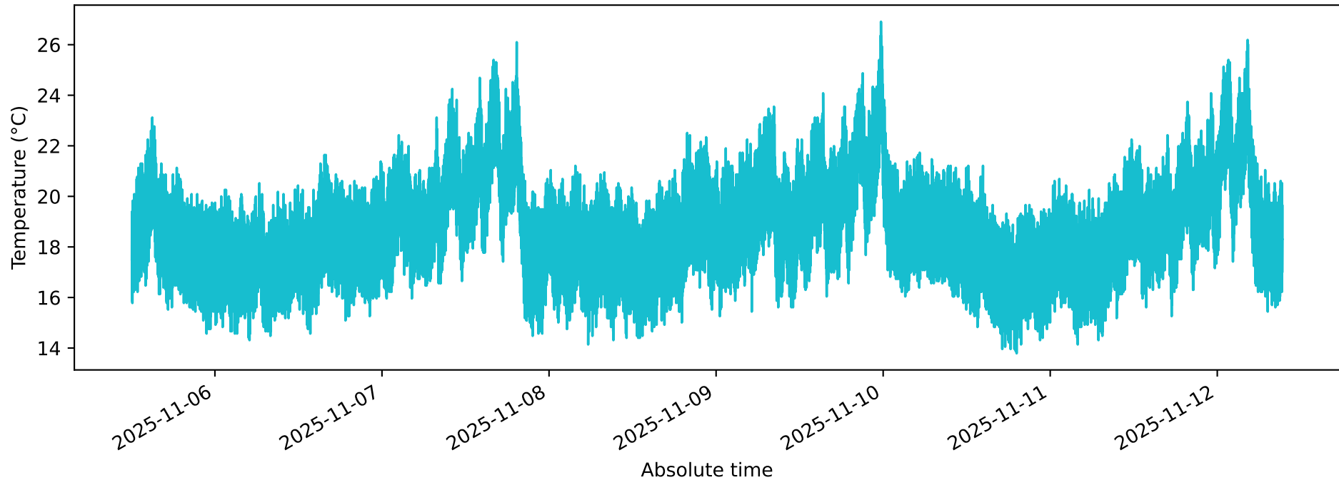
C_LFP_REPT_1_150_0043_temperature - T_4
