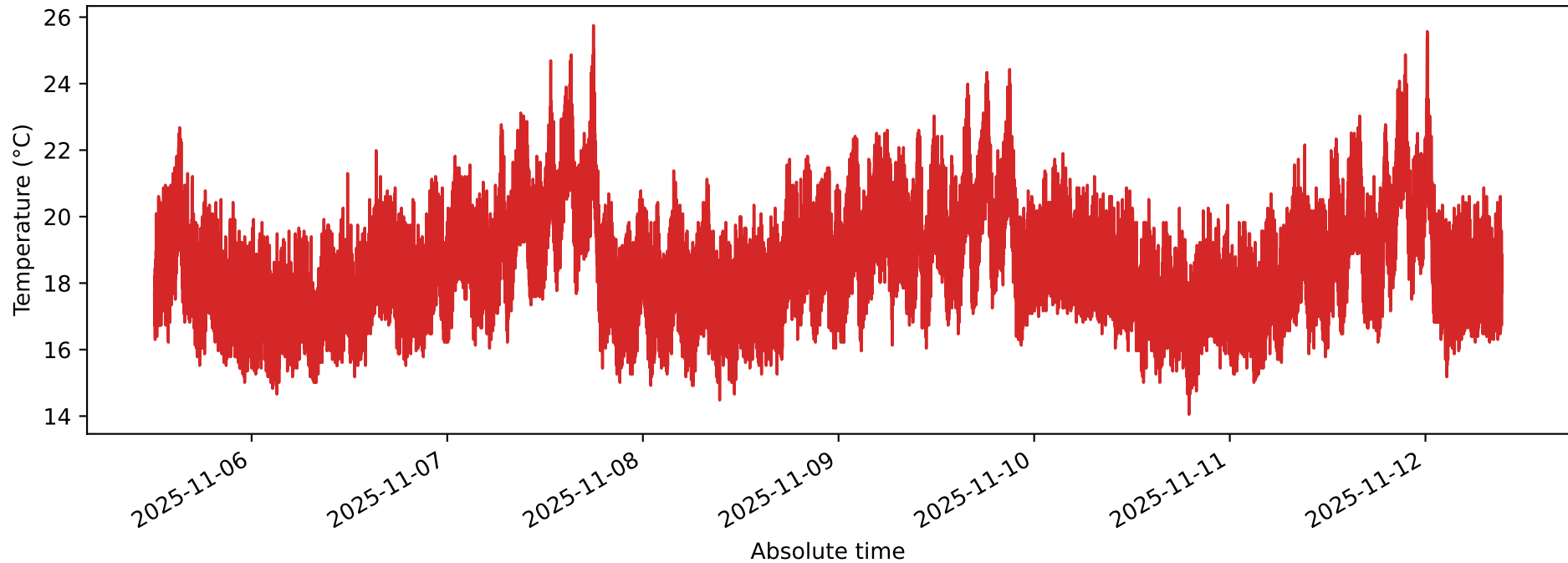
C_LFP_REPT_1_150_0080_temperature - T_2
