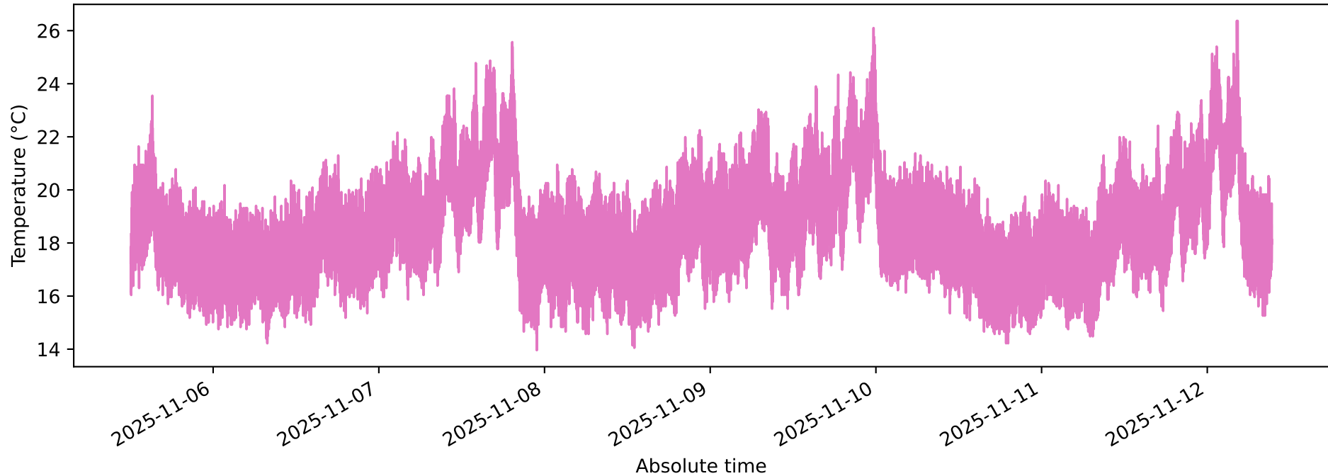
C_LFP_REPT_1_150_0043_temperature - T_3
