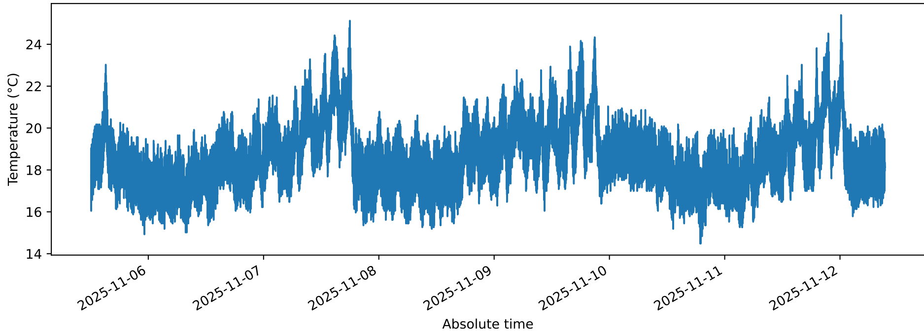
C_LFP_REPT_1_150_0080_temperature - T_1
