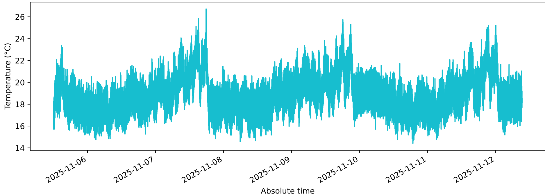
C_LFP_REPT_1_150_0080_temperature - T_4
