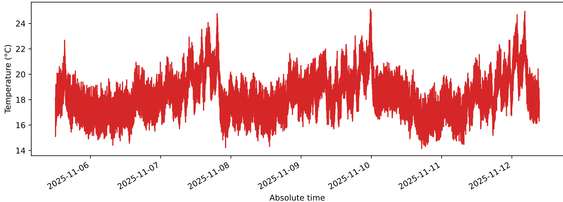
C_LFP_REPT_1_150_0043_temperature - T_2
