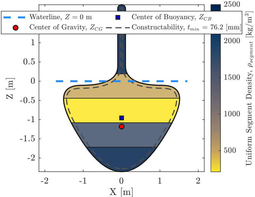
Stage 2: Modular Precast Construction
