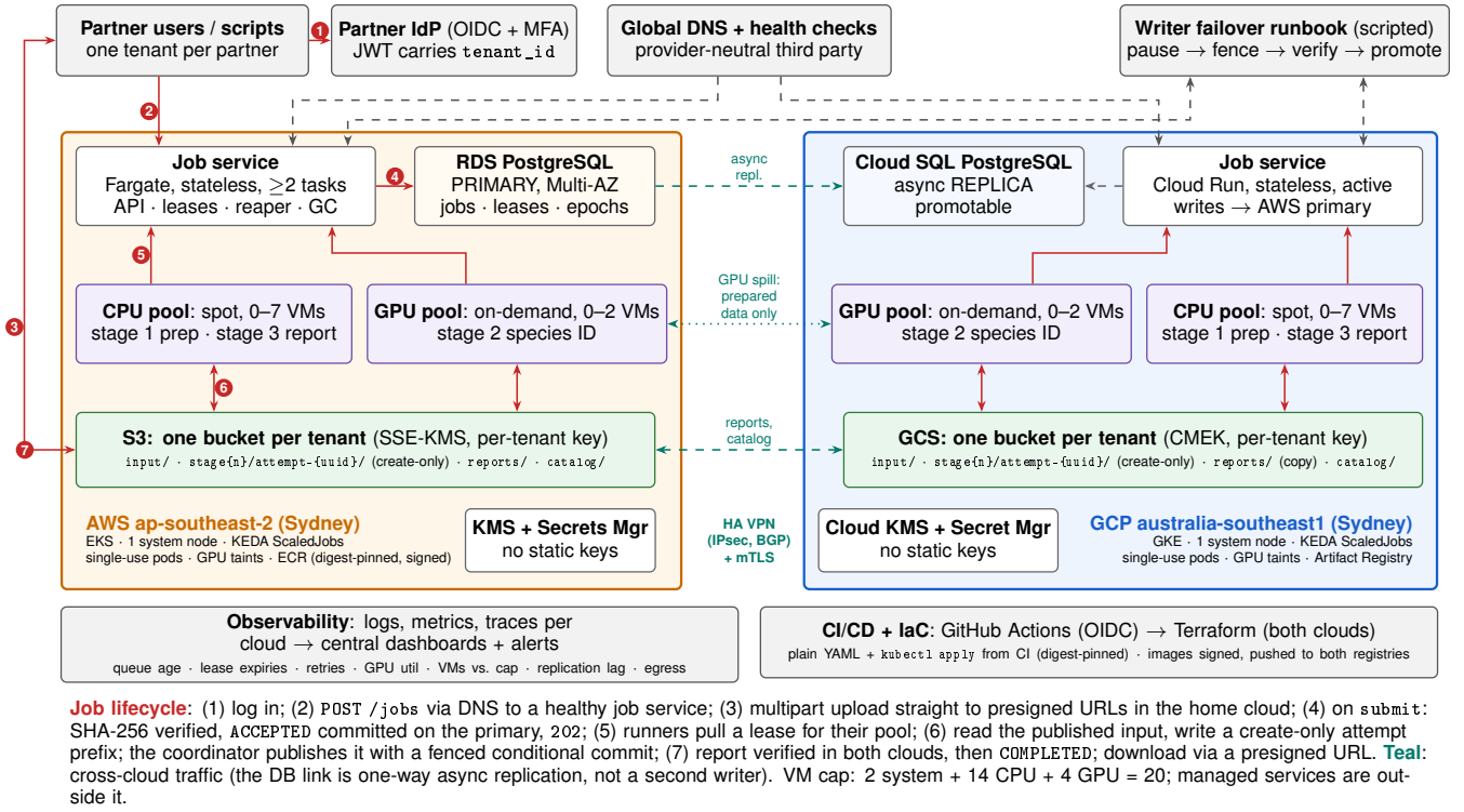
Figure 1: Architecture. Red numbers follow one job; teal links are the only cross-cloud traffic.
