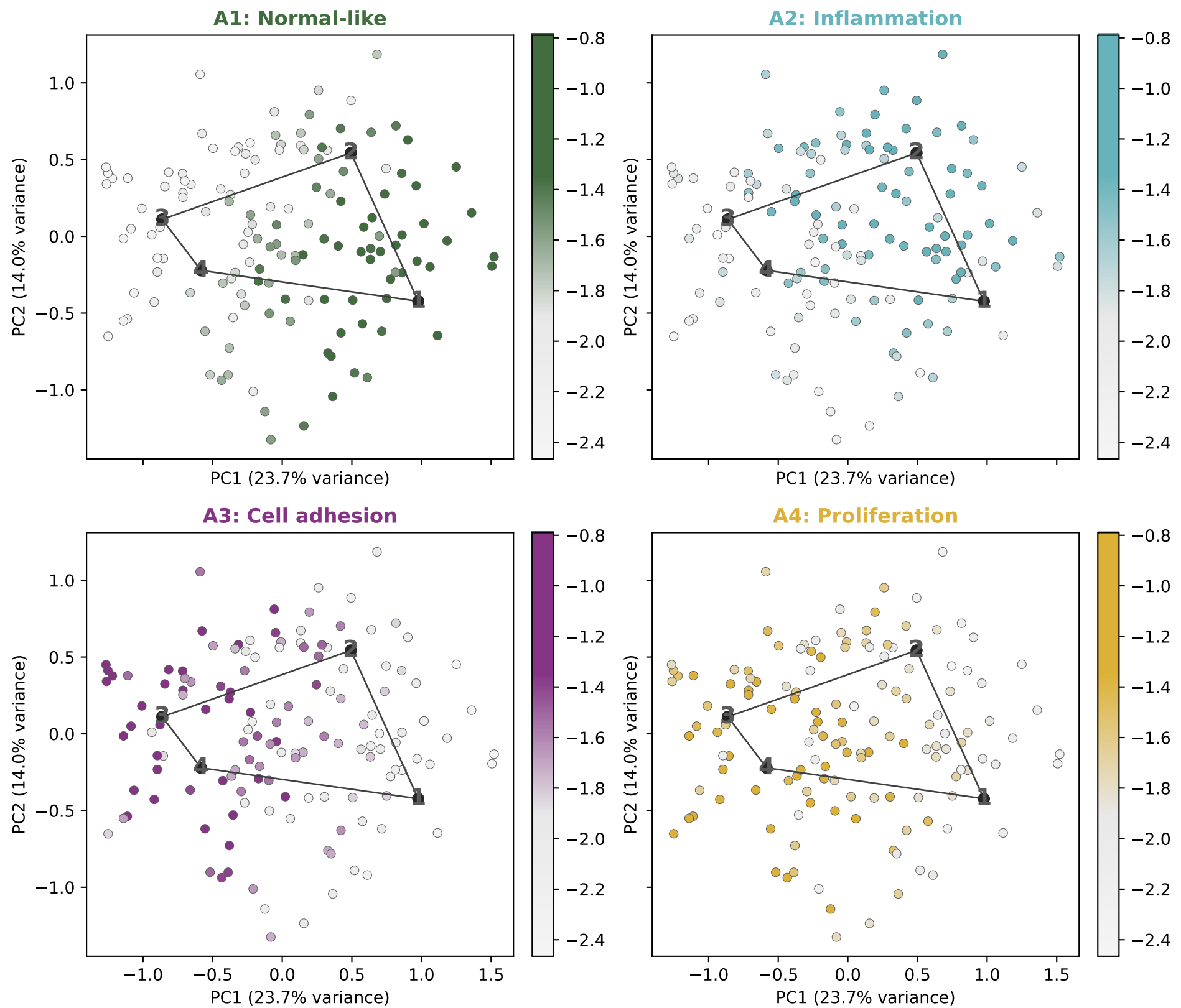
Fig 3A: NCBI-count voom GSVA \rightarrow author XC (PC1 flipped)
