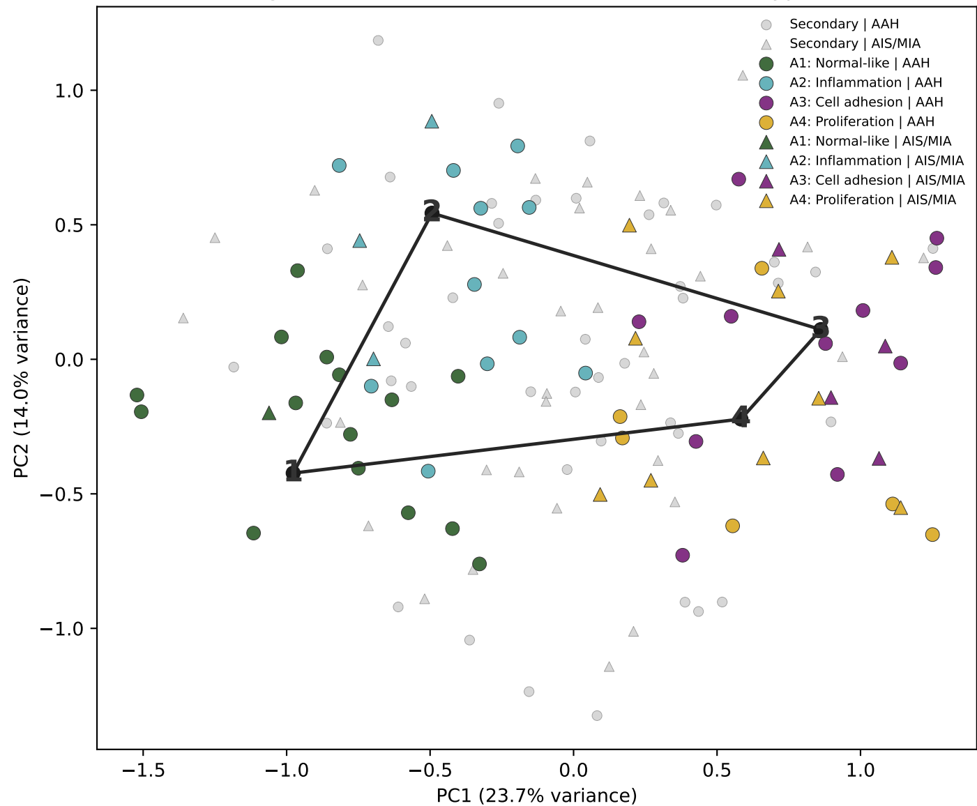
Fig 3B: NCBI-count voom + author-fixed archetypes
