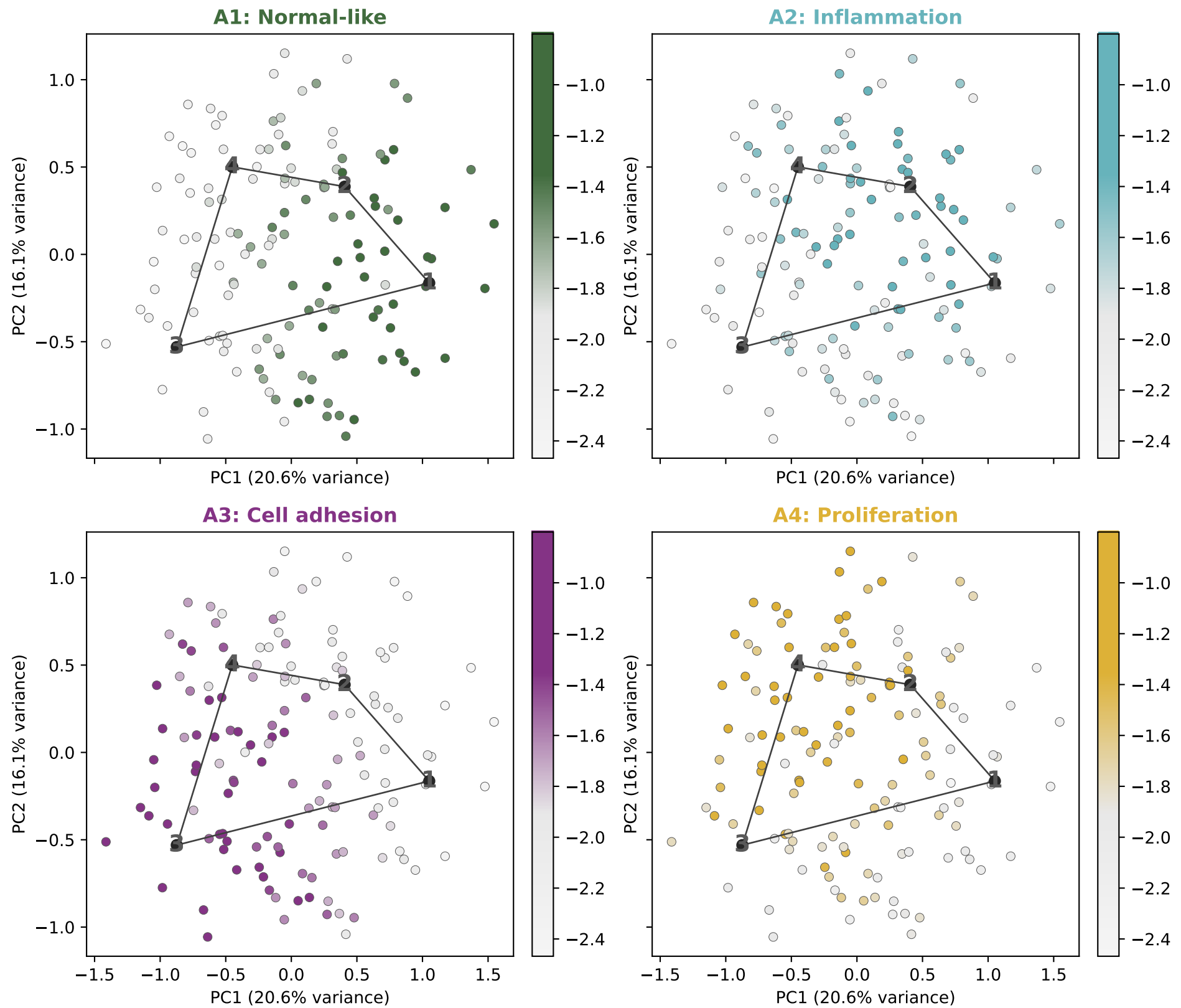
Fig 3A: author XC + v2 GSVA (PC1 flipped to paper side)
