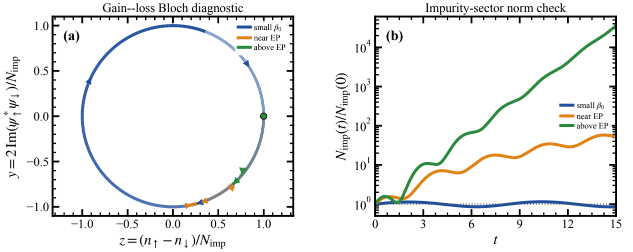
FIG. S1. Gain-loss Bloch diagnostic for the impurity sector. Panel (a) shows the normalized (z, y) trajectory for representative values of \beta_0 below, near, and above the EP. Below the EP the normalized co-decaying trajectory remains close to the unbroken relative-kernel orbit, while close to and beyond the EP the trajectory is progressively distorted. Panel (b) tracks the impurity-sector norm N_{\text{imp}}(t)/N_{\text{imp}}(0) and shows that the above-EP trajectory acquires a strong late-time amplification, whereas the below-EP and near-EP traces remain well controlled over the plotted time window.
