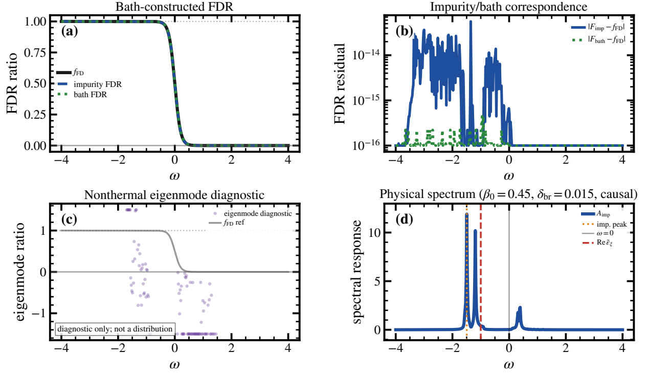
FIG. S7. Bath-controlled fluctuation-dissipation and spectral checks. The uniform reference is \epsilon_\xi = -U/2 = -1 , U = 2 , and T_b = 0.1 . Panels (a) and (b) verify the physical construction G_{\text{phys}}^< = G^R \Sigma_{\text{bath}}^< G^A = f_{\text{FD}}(G^A - G^R) with maximum residual 5.61 \times 10^{-14} at \delta_{\text{br}, \text{FDR}} = 10^{-3} . Panel (c) displays the distinct eigenmode occupation ratio only as a nonnormality diagnostic; it is not used in the saddle equations. Panel (d) shows the physical impurity spectral response with \delta_{\text{br}} = 0.015 . Any negative signed response in the broken relative-kernel continuation is classified as a causality diagnostic rather than a positive density of states.
