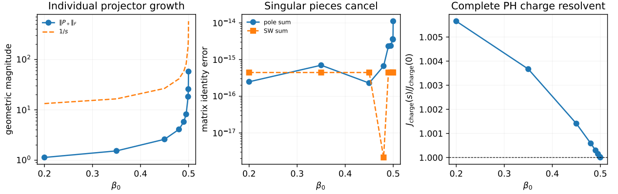
FIG. S3. Biorthogonal-projector and finite- U resolvent checks. Panel (a) shows the growth of an individual normalized projector and the artificial 1/s factor on the pre-EP side. Panel (b) verifies numerically that the two-projector pole sum equals the direct matrix resolvent and that the two virtual charge sectors equal the closed Schrieffer–Wolff resolvent; the plotted discrepancies are numerical roundoff. Panel (c) shows the complete particle–hole charge factor normalized to its EP limit. It remains finite and approaches unity although each projector grows. These checks exclude an independent Petermann or Z^{\text{bio}} multiplier from the Green function and screening estimate.
