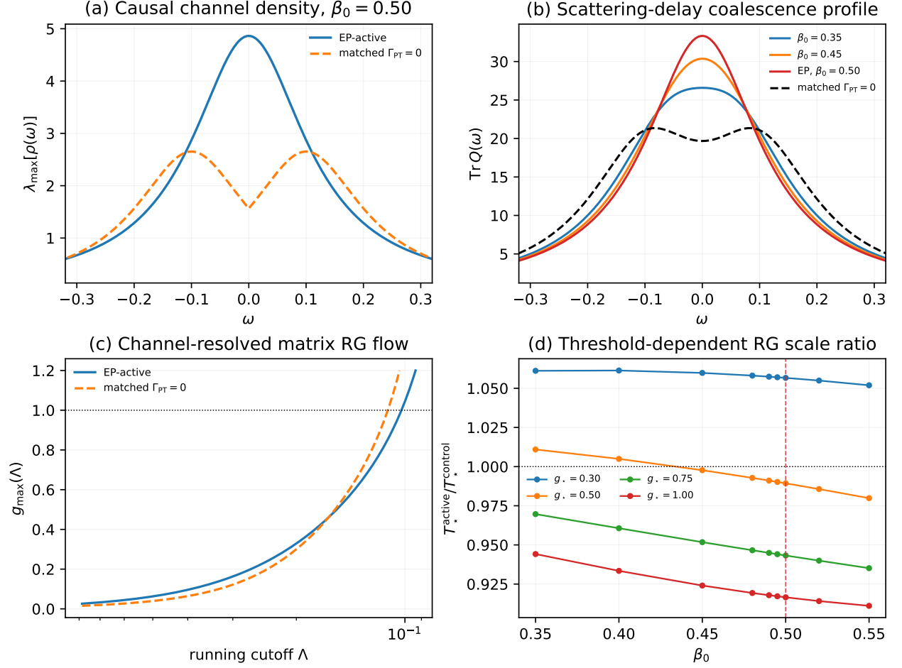
FIG. S6. Causal scattering and channel-resolved RG support. The conservative fixed- W validation uses the complete positive channel density from G^R and G^A , with \Gamma_0 = 0.12 and unit charge gap. Panel (a) compares the largest causal channel-density eigenvalue at \beta_0 = 0.50 with the matched \Gamma_{PT} = 0 control. Panel (b) gives the Wigner–Smith trace; the passive Fisher–Lee matrix is unitary to 1.33 \times 10^{-15} and \text{Tr}Q(0) = 4/\Gamma_0 = 33.3333 at the EP. Panels (c) and (d) show that the EP-active exchange eigenvalue is initially larger, but its threshold-scale ratio crosses below the control before strong coupling. This supports bounded pre-EP weak-flow amplification, not an enhanced thermodynamic Kondo temperature.
