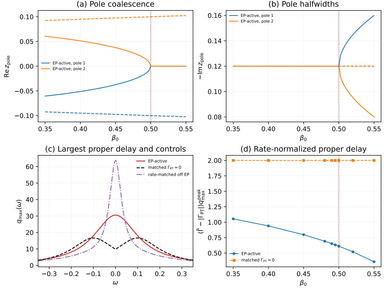
FIG. S4. Causal Smith-delay validation and adverse controls. Panel (a) tracks the analytic pole pair to the exact core EP at \beta_0 = 0.50 . Panel (b) shows the two passive halfwidths: they remain positive throughout the retained window and split only on the relative-broken side. Panel (c) compares the largest proper-delay peak with a Hermitian control matched by total rate and with an off-EP rate-matched kernel ( D = 0.05 ); the latter exceeds the EP peak. Panel (d) normalizes the largest proper delay by the slowest rate and likewise shows no independent EP enhancement. Together with the unitarity and trace-delay checks in App. I, these controls establish the Smith profile as a causal coalescence/linewidth fingerprint, not a Kondo-scale multiplier.
