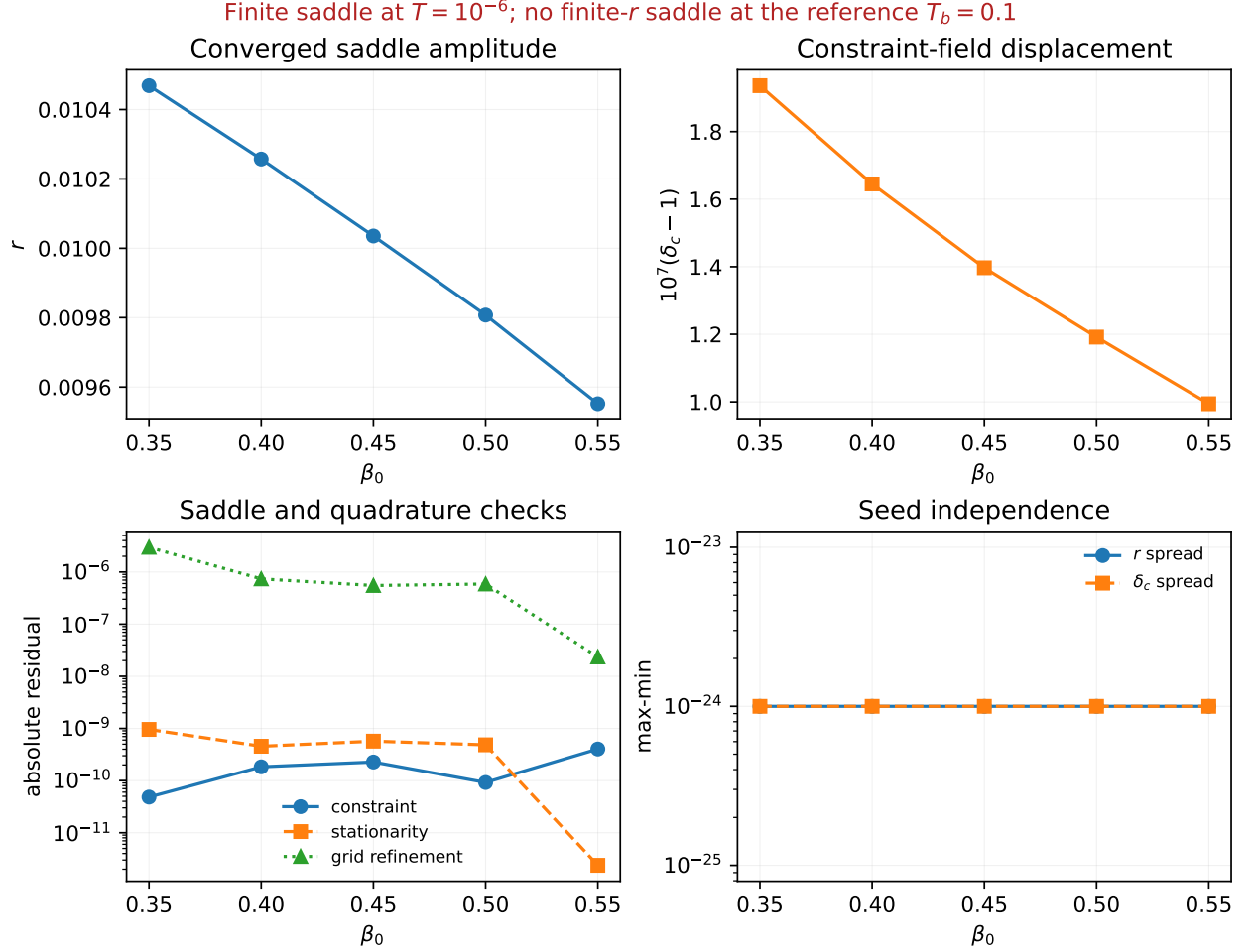
FIG. S2. Low-temperature U \rightarrow \infty saddle and numerical acceptance tests. At T_b = 10^{-6} , panel (a) shows the converged amplitude r and panel (b) the constraint-field displacement over 0.35 \leq \beta_0 \leq 0.55 . Panel (c) reports the final constraint, stationarity, and grid-refinement residuals; panel (d) shows that real, negative-real, and complex initial boson seeds converge to the same gauge-fixed solution. The complete sandwich construction satisfies charge continuity to 3.94 \times 10^{-23} . The title records the distinct result at the manuscript reference temperature: the same closure has no finite- r branch at T_b = 0.1 . The figure therefore validates the low-temperature saddle and the exact core-EP scaling, but does not claim finite-temperature condensate enhancement.
