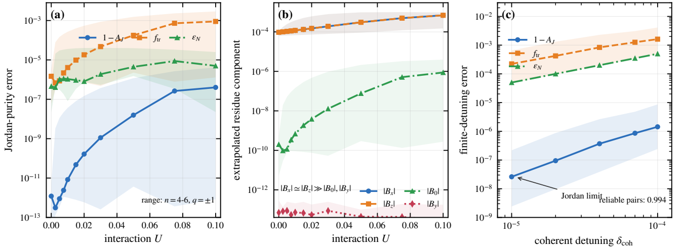
FIG. S8. Finite- U Jordan transition-residue audit for the scalar-hybridization NRG control. (a) Zero-detuning extrapolations of the alignment error 1 - A_J , trace fraction f_{\text{tr}} , and nilpotent mismatch \epsilon_N . Curves are medians and bands are the full range over iterations n = 4-6 and charge sectors q = \pm 1 . (b) Pauli components of the extrapolated double-pole coefficient B : |B_x| \simeq |B_z| \gg |B_0|, |B_y| , as required by N_{\text{EP}} = \Delta_{\text{eff}} \sigma_z + i \Gamma_{\text{PT}} \sigma_x . (c) Direct finite-detuning convergence; curves are medians and bands are the 16th–84th percentile over U , iteration, and tracked sector. The reliable-pair fraction is 0.994. Parameters are \Lambda = 3 , z = 0.5 , N_{\text{keep}} = 320 , r = 1 , \beta_0 = 0.50 , \Delta_{\text{eff}} = \Gamma_{\text{PT}} = 0.10 , and 0 \leq U \leq 0.10 . The figure establishes persistence of the nilpotent matrix-residue direction; it does not establish pole coalescence, a universal interaction law, a thermodynamic Kondo scale, or a phase boundary.
