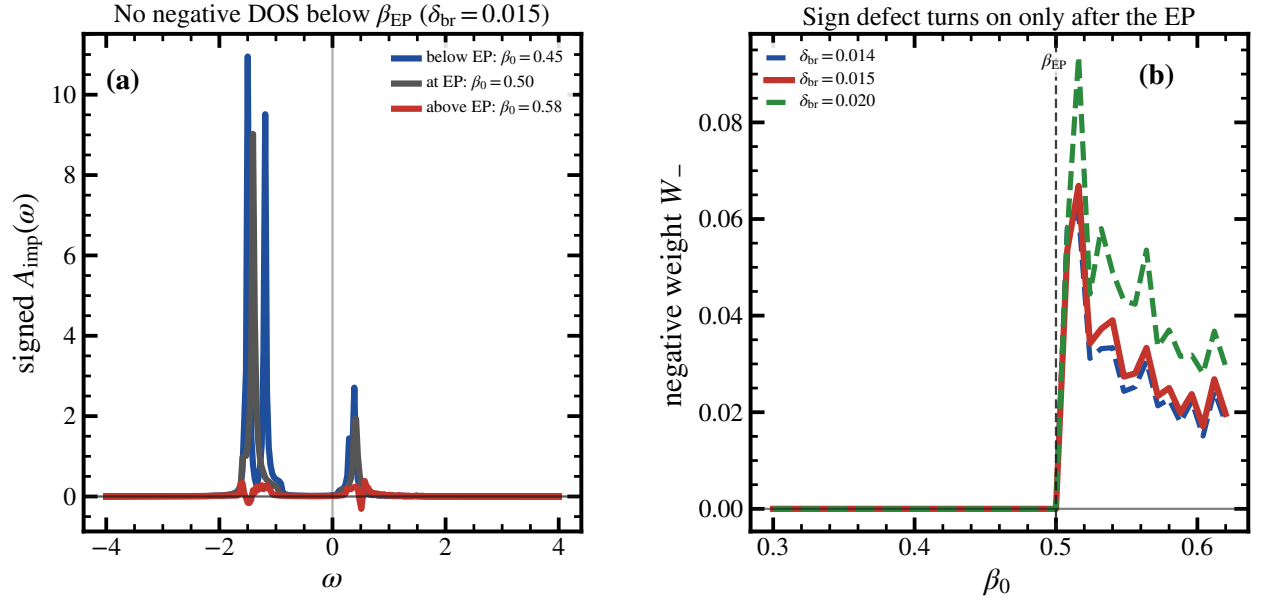
FIG. S5. Onset of negative signed spectral weight only beyond the EP. Panel (a) compares the signed impurity spectral response below the EP ( \beta_0 = 0.45 ), at the EP ( \beta_0 = 0.50 ), and above the EP ( \beta_0 = 0.58 ) for \delta_{\text{br}} = 0.015 . No negative signed relative-kernel response appears below the EP, while a sign defect emerges only on the PT-broken side. Panel (b) quantifies the integrated negative weight \mathcal{W}^- for \delta_{\text{br}} = 0.014, 0.015, 0.020 and shows that it remains zero up to the EP and turns on only after \beta_{0,\text{core}}^{\text{EP}} = 0.50 . This confirms that the negative signed response is an above-EP effect rather than a broadening artefact.
