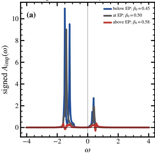
No negative DOS below \beta_{\text{EP}} ( \delta_{\text{br}} = 0.015 )
