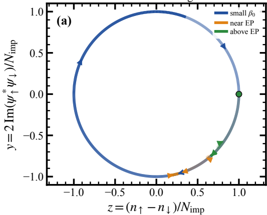
Gain--loss Bloch diagnostic
