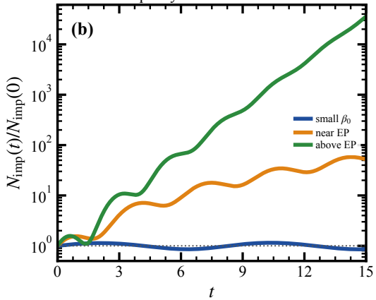
Impurity-sector norm check
